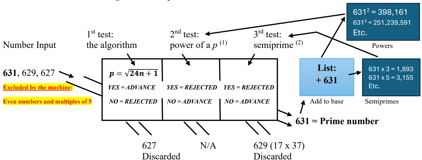
Diagram 1: The prime number detection machine
