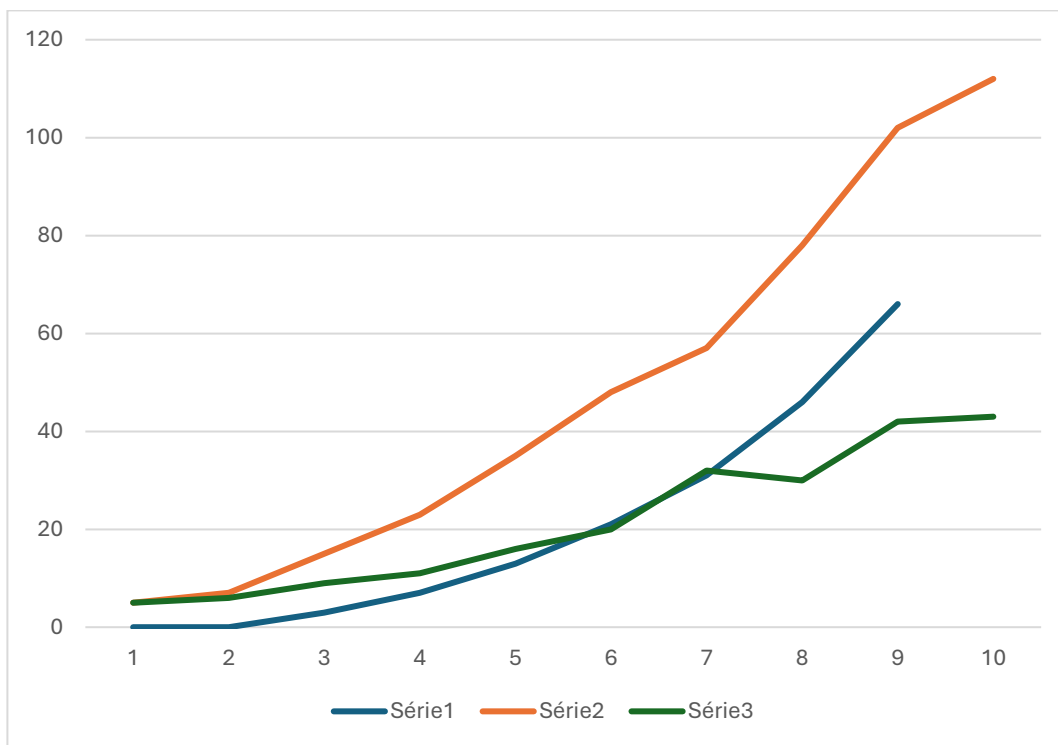
Diagram 3: Comparison between the number of false positives, semiprimes and primes situated between the squares of a twin prime pair
