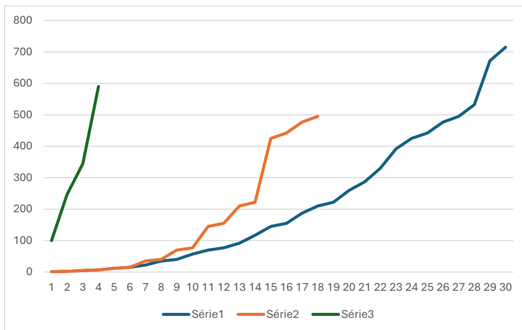
Diagram 4: Multiplicative factors of number 24 associated with the squares of primes, twin primes and false positives
