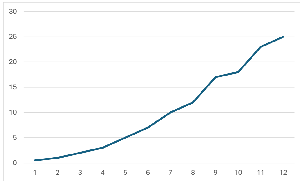
Diagram 5 : Multiplicative factors of the number 24 associated with the difference between the squares of two successive pairs of twin primes
