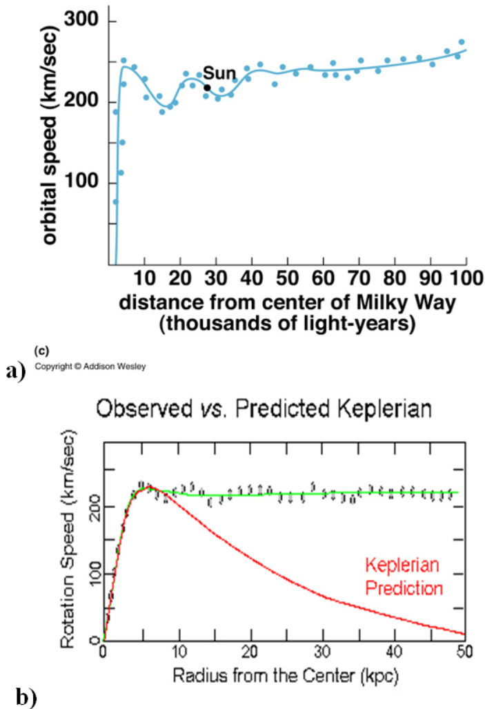
Fig.2. Dependencies of velocity of rotation of astronomical objects on the distance to gravity center: (a) our Milky Way galaxy [54, 55], (b) comparing to prognosed Keplerian velocities [53, 56]).
