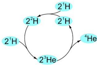
Fig.11 pp-I branch. {}^1\text{H} is converted to {}^2\text{H} , then to {}^3\text{He} and finally to {}^4\text{He} by proton capture.
