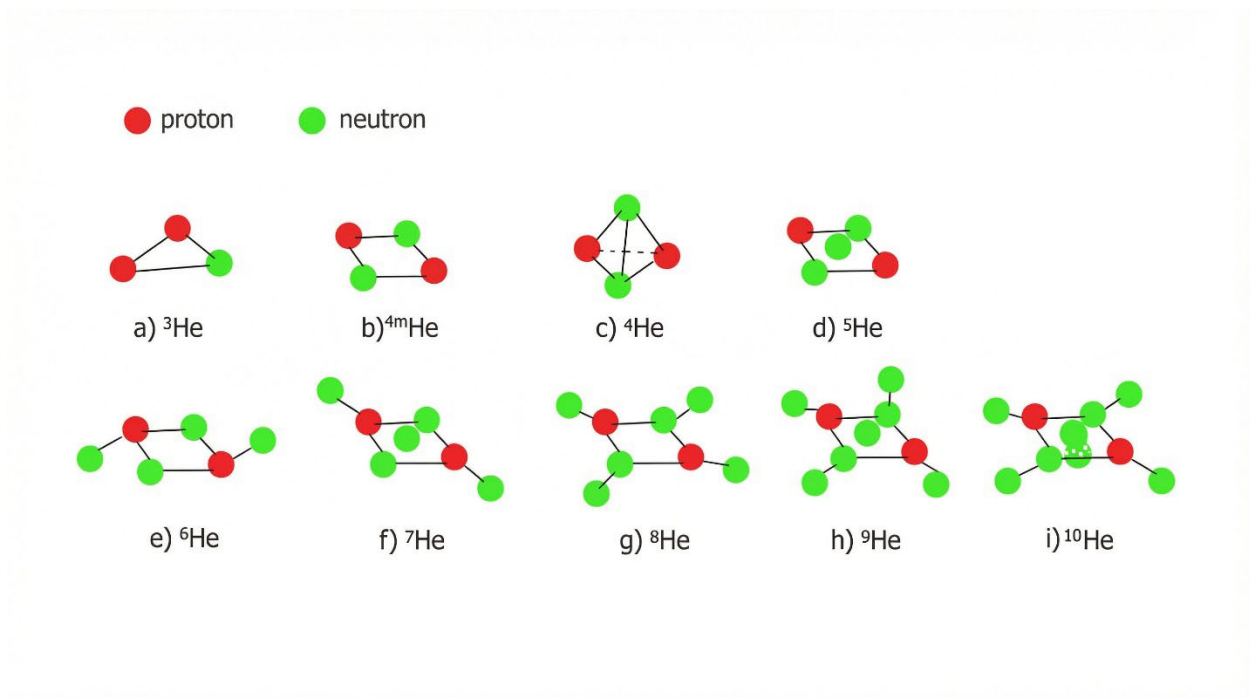
Fig.15 Binding structures of He isotopes.
