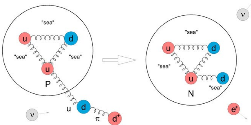
Fig. 5 \beta^+ decay. When a neutrino interacts with a pion, the excited pion may decay into an electron and a positron. The electron can be absorbed by the proton's core, resulting in the conversion of the proton into a neutron, while the positron moves away from the nucleus.
