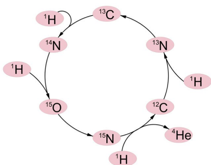
Fig.12 The CNO cycle consists of four proton-capture fusion reactions and two \beta^+ decays.
