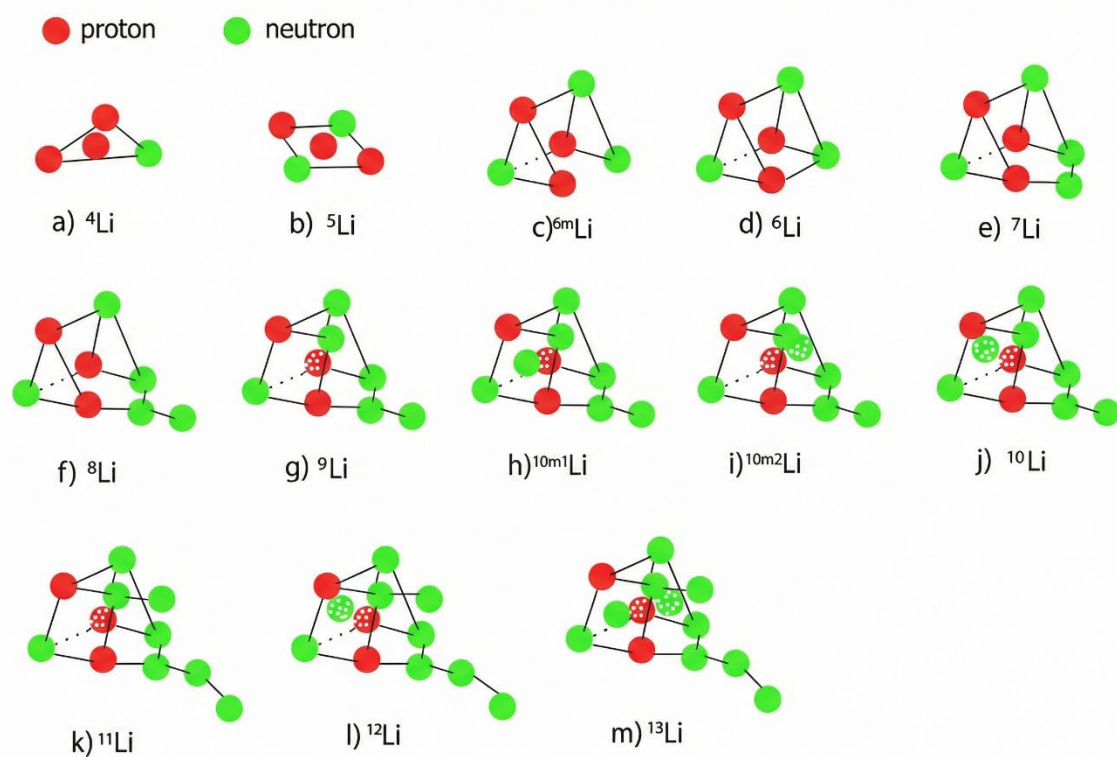
Fig.16 Binding structures of Li isotopes.
