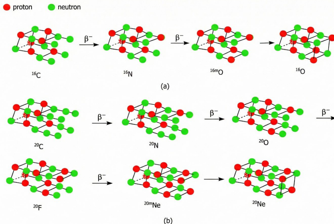
Fig. 9| Beta decay studies have shown that ^{16}\text{O} and ^{20}\text{Ne} have transition isomers, ^{16m}\text{O} and ^{20m}\text{Ne} .
