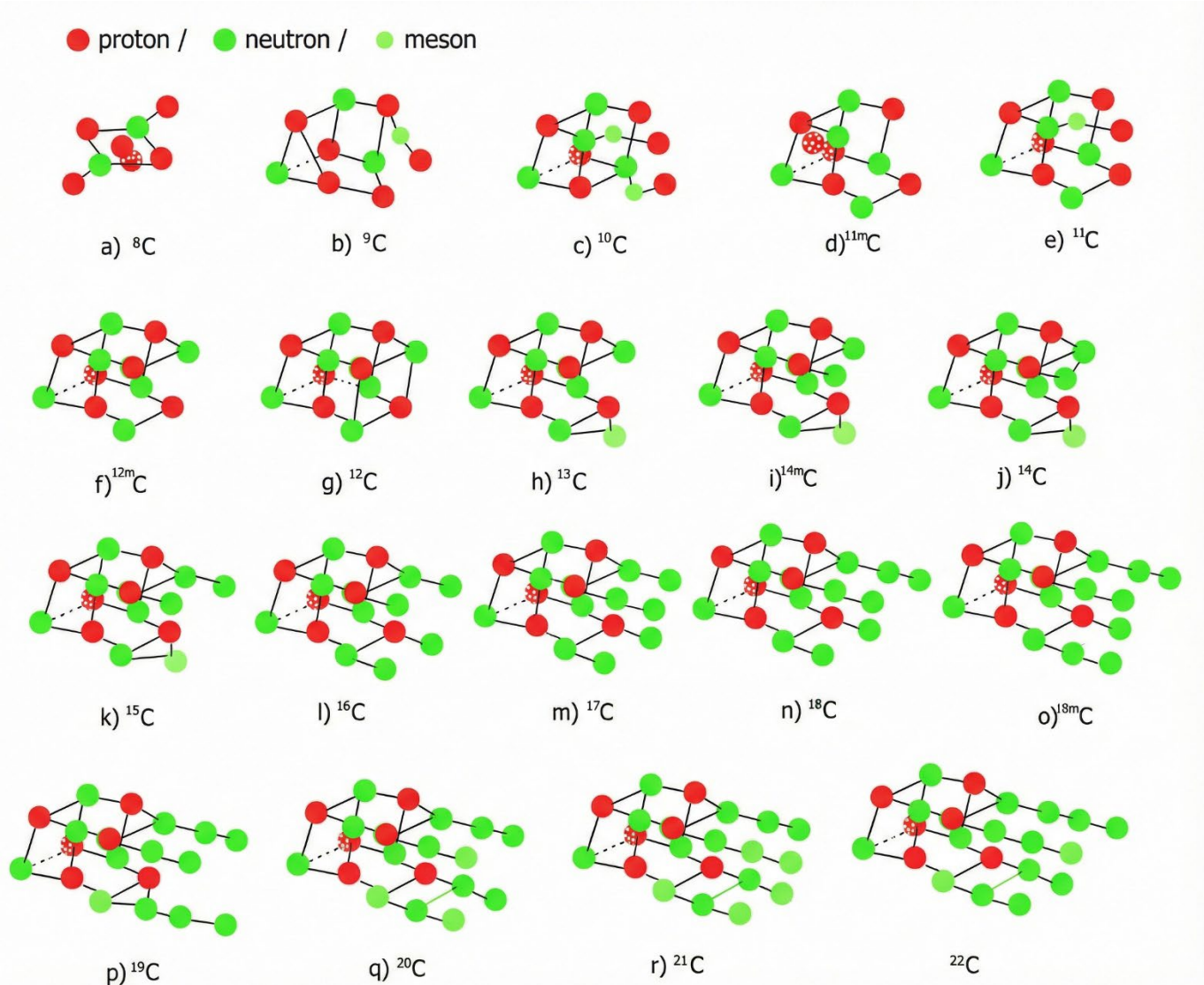
Fig.19 Binding structures of C isotopes
