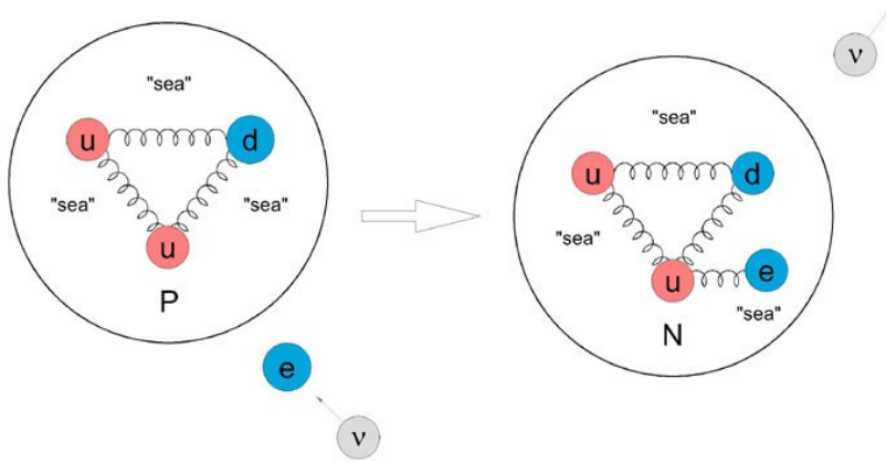
Fig. 6 | Neutrino-induced Electron Capture. In a proton-rich and electron-rich atom, an electron is knocked by a neutrino and captured by the proton, then bound to the core by a gluon, which makes the proton transmute to a neutron.
