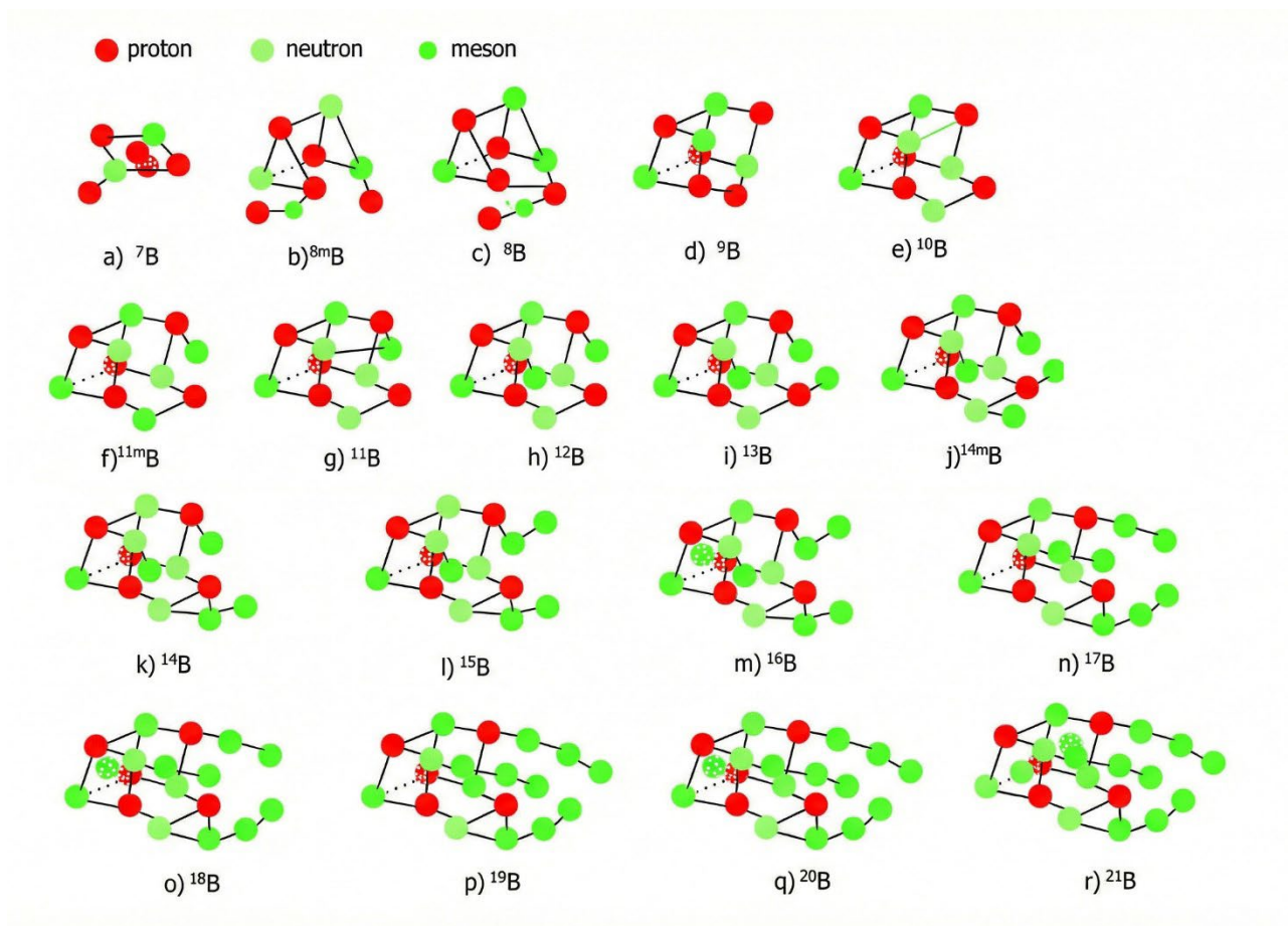
Fig.18| Binding structures of B isotopes.
