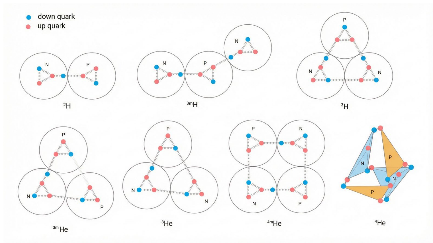
Fig. 7|Basic nuclides and their internal binding structures. Nucleons are bound by Direct Gluon Bonds between down quark and up quark of their core structures.
