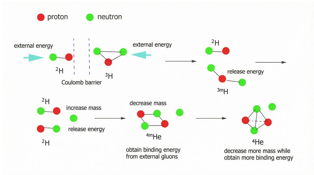
Fig.10| Several processes in the D-T reaction involve changes in binding energy.
