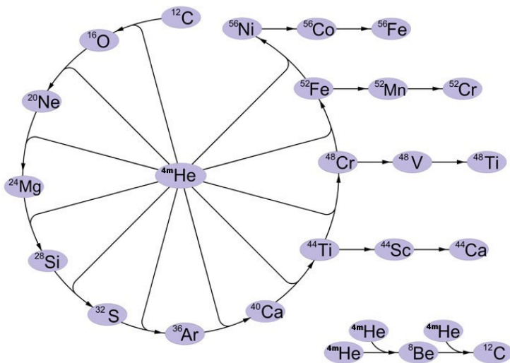
Fig.13|Alpha-process: all participating nuclides possess an equal number of protons and neutrons, with their atomic numbers being multiples of four.
