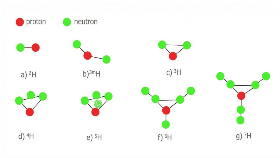
Fig.14 Binding structures of H isotopes.
