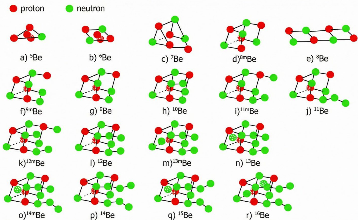
Fig.17 Binding structures of Be isotopes.
