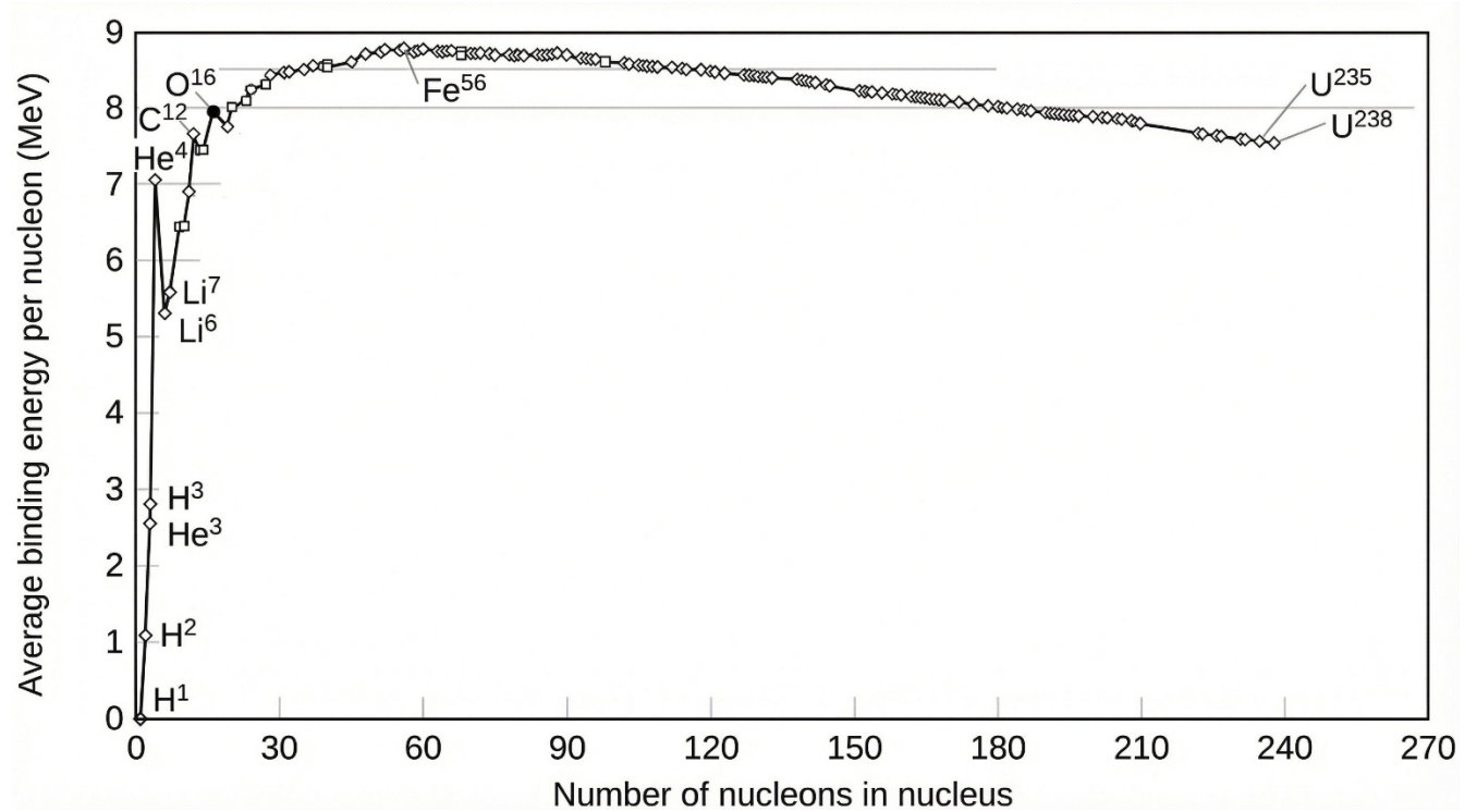
Fig.8| Binding energy per nucleon. Source: Wikipedia ( https://en.wikipedia.org/wiki/Nuclear_binding_energy ). Data available from the NuDat 2 database ( 221 ).
