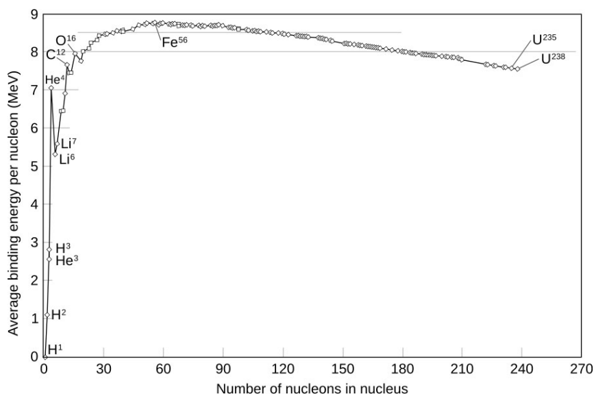
Fig.12. Binding energy per nucleon. Source: Wikipedia ( https://en.wikipedia.org/wiki/Nuclear_binding_energy ). Data available from the NuDat 2 database.(211).
