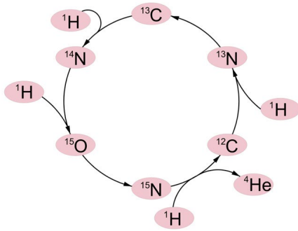
Fig.16 |The CNO cycle consists of four proton-capture fusion reactions and two \beta^+ decays.
