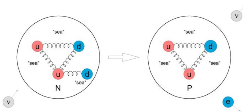
Fig.5| \beta^- decay. A neutron interacts with a neutrino, resulting in the transformation of the neutron into a proton as one of its down quarks is removed. The neutrino experiences elastic scattering, altering its trajectory and continuing onward with reduced kinetic energy.
