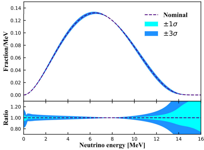
Fig. 10 | ^8\text{B} and hep \nu_e spectrum with the shape uncertainties. Figure taken from Ref.( 156 ).
