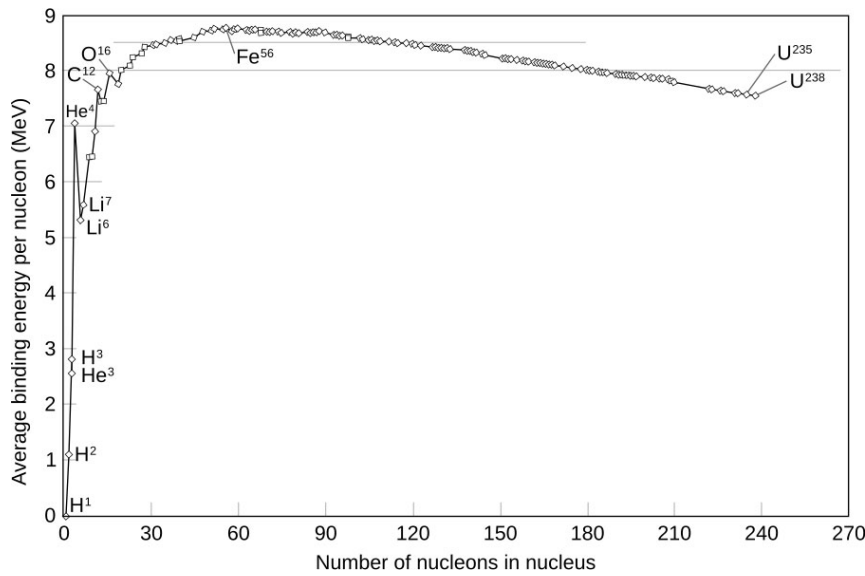
Fig.12. Binding energy per nucleon. Source: Wikipedia ( https://en.wikipedia.org/wiki/Nuclear_binding_energy ). Data available from the NuDat 2 database.(199).
