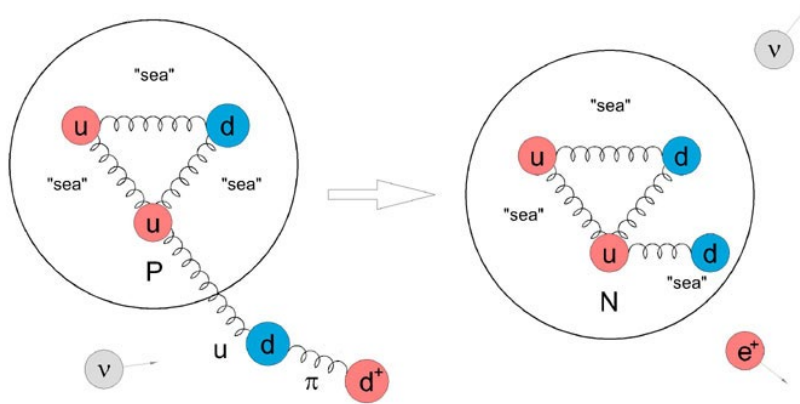
Fig. 6 \beta^+ decay. When a neutrino interacts with a pion, the excited pion may decay into an electron and a positron. The electron can be absorbed by the proton's core, resulting in the conversion of the proton into a neutron, while the positron moves away from the nucleus.
