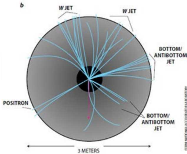
Fig.4| t\bar{t} collision event. This was described as \bar{p}p \rightarrow t\bar{t} \rightarrow \bar{p}p \rightarrow t\bar{t} \rightarrow W^+W^- \bar{b}b .
