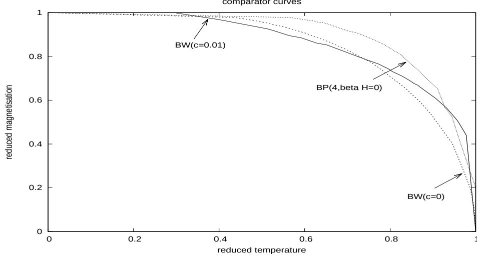
FIG. 28. Reduced magnetisation vs reduced temperature curves for Bragg-Williams approximation, in absence(dark) of and presence(inner in the top) of magnetic field, c = \frac{H}{\gamma\epsilon} = 0.01 , and Bethe-Peierls approximation in absence of magnetic field, for four nearest neighbours (outer in the top).
