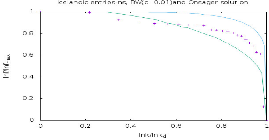
FIG. 2. Vertical axis is \frac{\ln f}{\ln f_{max}} and horizontal axis is \frac{\ln k}{\ln k_{lim}} . The + points represent the words of the Icelandic language, in bold(no supplement), with the fit curve being the Bragg-Williams curve, BW( c=0.01 ), in the presence of external magnetic field, H, with c = \frac{H}{\gamma\epsilon} = 0.01 . The uppermost curve is the Onsager solution.
