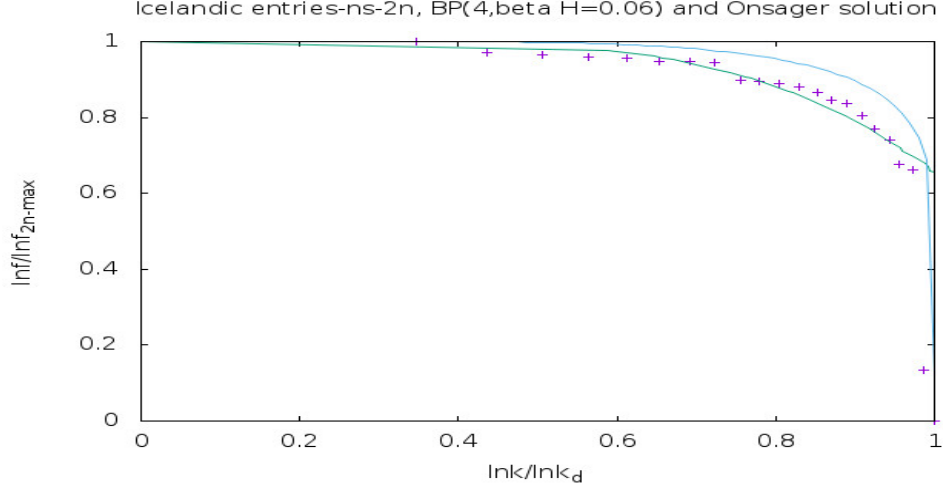
FIG. 4. Vertical axis is \frac{\ln f}{\ln f_{2n-max}} and horizontal axis is \frac{\ln k}{\ln k_{lim}} . The + points represent the words of the Icelandic language, in bold(no supplement), with the fit curve being the Bethe-Peierls curve with four nearest neighbours, in presence of little magnetic field, m=0.03 or, \beta H = 0.06 . The uppermost curve is the Onsager solution.
