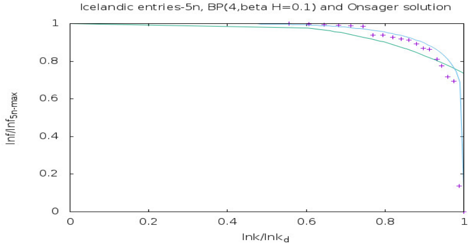
FIG. 18. Vertical axis is \frac{\ln f}{\ln f_{5n-\max}} and horizontal axis is \frac{\ln k}{\ln k_{lim}} . The + points represent the words of the Icelandic language, in bold, with the fit curve being the Bethe-Peierls curve with four nearest neighbours, in presence of little external magnetic field, m=0.05 or, \beta H = 0.1 . The uppermost curve is the Onsager solution.
