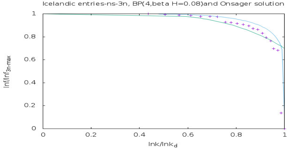
FIG. 5. Vertical axis is \frac{\ln f}{\ln f_{3n-max}} and horizontal axis is \frac{\ln k}{\ln k_{lim}} . The + points represent the words of the Icelandic language, in bold(no supplement), with the fit curve being the Bethe-Peierls curve with four nearest neighbours, in presence of little magnetic field, m=0.04 or, \beta H = 0.08 . The uppermost curve is the Onsager solution.
