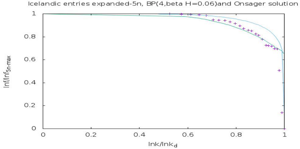
FIG. 27. Vertical axis is \frac{\ln f}{\ln f_{5n-max}} and horizontal axis is \frac{\ln k}{\ln k_{lim}} . The + points represent the words of the Icelandic language, in bold, in expanded Icelandic alphabet, with the fit curve being the Bethe-Peierls curve with four nearest neighbours, in presence of little external magnetic field, m=0.03 or, \beta H = 0.06 . The uppermost curve is the Onsager solution.
