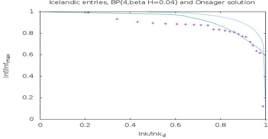
FIG. 13. Vertical axis is \frac{\ln f}{\ln f_{\max}} and horizontal axis is \frac{\ln k}{\ln k_{\lim}} . The + points represent the words of the Icelandic language, in bold, with the fit curve being the Bethe-Peierls curve with four nearest neighbours, in presence of little external magnetic field, m=0.02 or, \beta H = 0.04 . The uppermost curve is the Onsager solution.
