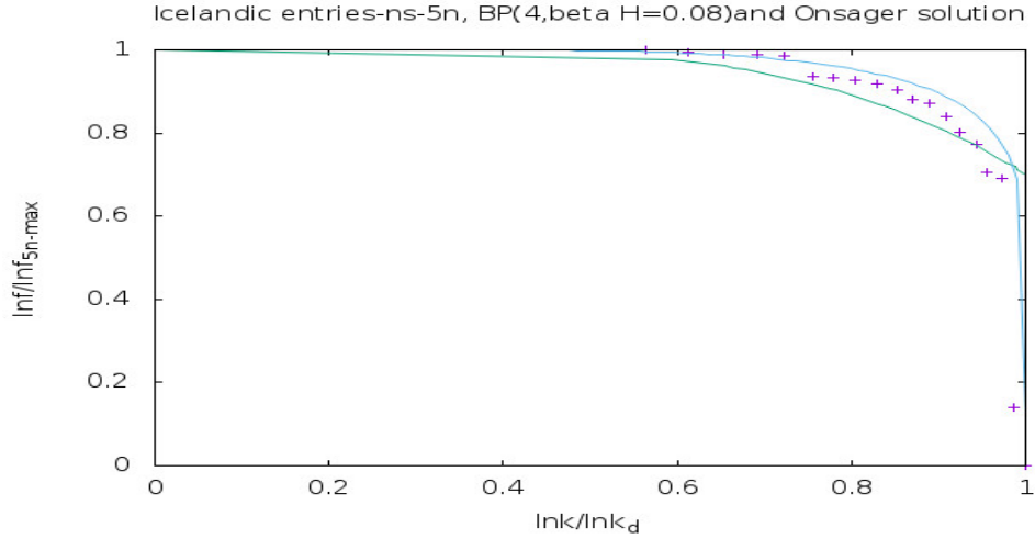
FIG. 7. Vertical axis is \frac{\ln f}{\ln f_{5n-max}} and horizontal axis is \frac{\ln k}{\ln k_{lim}} . The + points represent the words of the Icelandic language, in bold(no supplement), with the fit curve being the Bethe-Peierls curve with four nearest neighbours, in presence of little magnetic field, m=0.04 or, \beta H = 0.08 . The uppermost curve is the Onsager solution.
