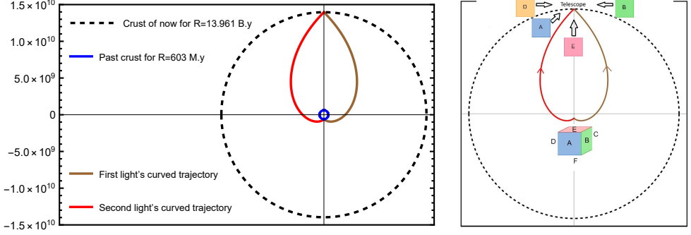
Figure 6: The position of the first mirror point relative to Earth within the four-dimensional sphere of the universe.
