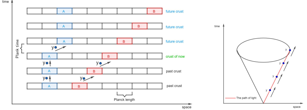
Figure 3: Illustration of the time mechanism for the space crust at the quantum scale and its comparison with Einstein's light cone.
