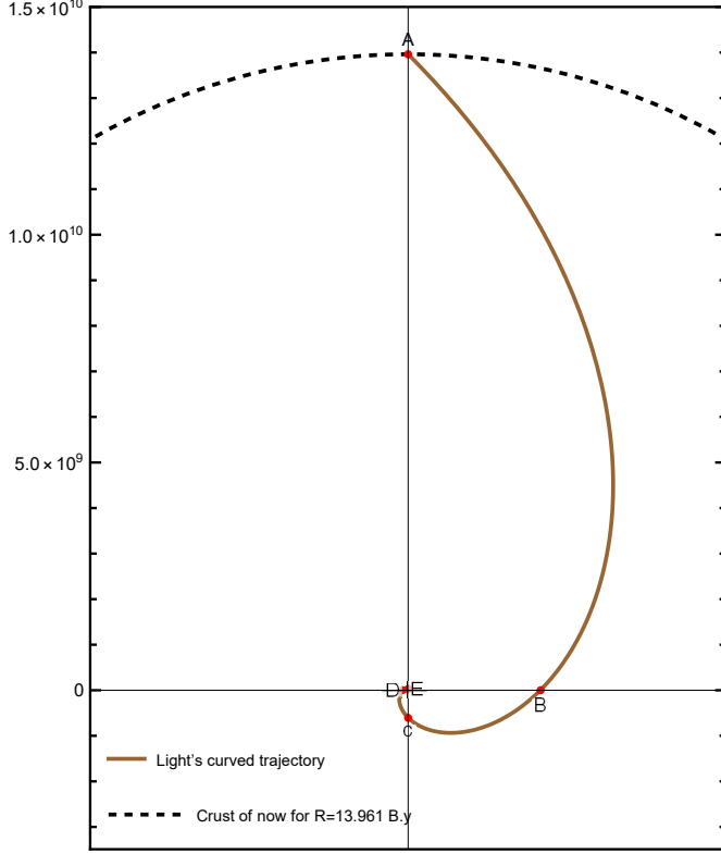
Figure 7: The positions of four points, each with a phase difference of \frac{\pi}{2} , during the final complete cycle of light reaching Earth within the four-dimensional sphere of the universe.
