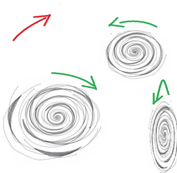
fig 1: „External Field Effect“: Three galaxies with different rotational directions of their own, but which all rotate together in the same cluster in the same direction. For stars on the edge of large galaxies, the direction of the cluster rotation has just as great an impact as the rotation of their own galaxy.
