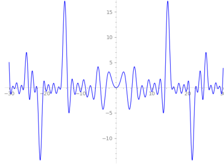
Fig. 11 Graph of Z -function along [Analytically normalized] \Re(s) = \frac{1}{2} -critical line for -\infty < t < \infty depicting UNIQUE nontrivial zeros spectrum for Elliptic curve LMFDB label 389.a1 [with non-zero Analytic rank of 2]. Note **Line Symmetry of vertical y -axis and trajectory intersecting Origin point. Integral points are (-2, 0), (-2, -1), (-1, 1), (-1, -2), (0, 0), (0, -1), (1, 0), (1, -1), (3, 5), (3, -6), (4, 8), (4, -9), (6, 15), (6, -16), (39, 246), (39, -247), (133, 1539), (133, -1540), (188, 2584), (188, -2585) .
