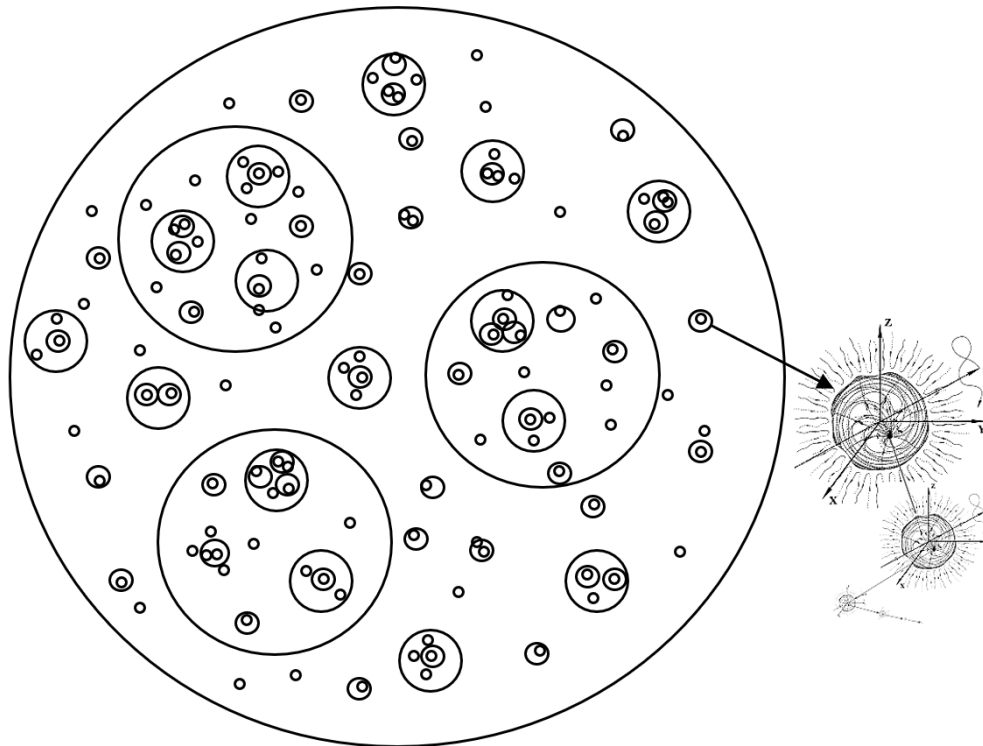
Fig. 10. Illustration of a hierarchical cosmological model consisting of a set of spherical vacuum formations (corpuscles) differently nested into each other
