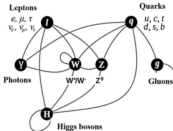
Fig. 9. Elements of the Standard Model of Elementary Particles
