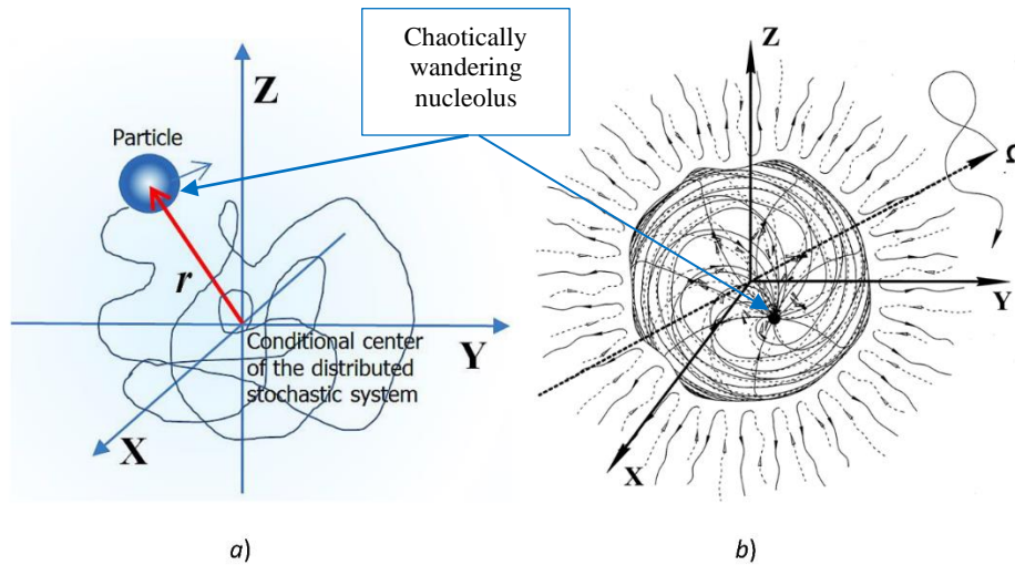
Fig. 4. A simplified representation of the inner nucleolus as a solid particle with a radius r_7 \sim 10^{-24} cm, which wanders chaotically in the vicinity of the center of the core of an elementary particle (in particular, an "electron") due to random force effects from the fluctuating elastic-plastic medium and elastic forces tending to return the nucleolus to the conditional center of the stochastic system under consideration.
