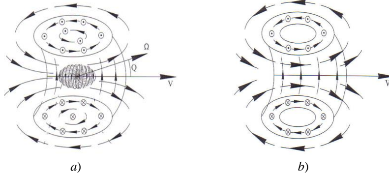
Fig. 6. a) The core and outer shell of a moving "electron" rotate around the direction of its motion. b) A "neutrino" is a toroidal vortex disturbance of the vacuum without a core in the middle, moving at a speed close to the speed of light.
