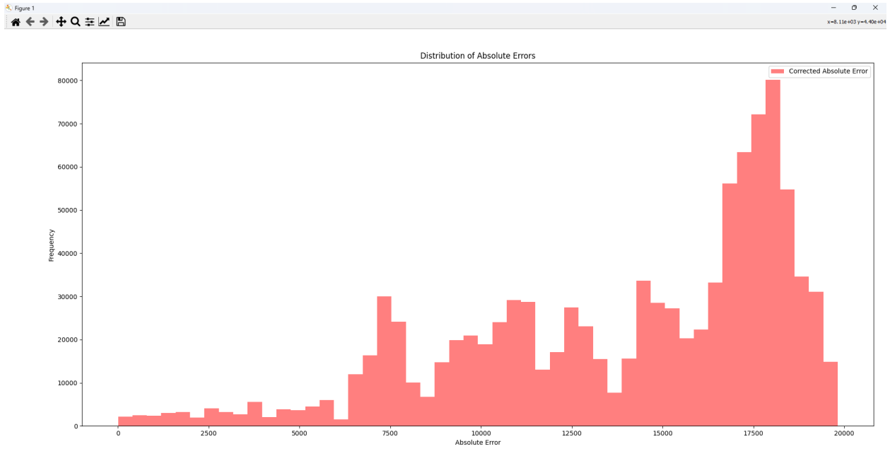
Figure 5: Histogram Analysis of Frequency vs Magnitude of Errors for New Equation
