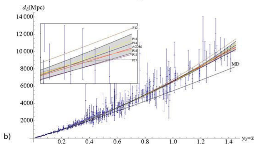
Fig. 3. Dependencies of distances to astronomical objects on the redshift of radiation of astronomical objects z :
