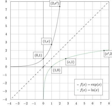
8 The natural logarithm function \log_e x or \ln(x) and natural exponential function \exp(x) or e^x . The graphs of \log_e x and its inverse e^x are symmetric with respect to line y = x thus geometrically denoting diagonal symmetry of these two functions; viz, \ln(e^x) = x and e^{\ln(x)} = x .
