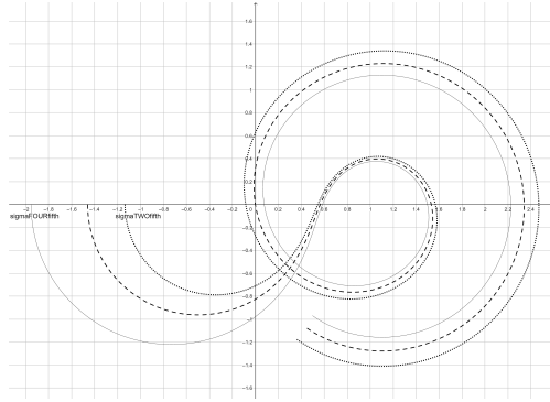
10 Simulated dynamic trajectories showing Origin intercept points when \sigma = \frac{1}{2} and virtual Origin intercept points when \sigma = \frac{2}{5} and \sigma = \frac{4}{5} . Horizontal axis: Re\{\zeta(\sigma + it)\} , and vertical axis: Im\{\zeta(\sigma + it)\} . Total presence of all Origin intercept points at the [static] Origin point. Total presence of all virtual Origin intercept points as additional negative virtual Gram[y=0] points on the x-axis (e.g. when using \sigma = \frac{2}{5} value) at the [infinitely many varying] virtual Origin points; viz, these negative virtual Gram[y=0] points on the x-axis cannot exist at the solitary Origin point since the two trajectories form two colinear lines (or co-lines); viz, two parallel lines that never cross over.
