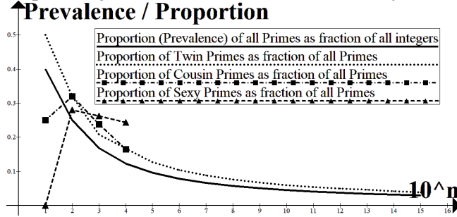
9 Proportion (Prevalence) of Twin primes, Cousin primes [as partial calculations] and Sexy Primes [as partial calculations] with Proportion (Prevalence) of all Primes included. These Proportions (Prevalences) are essentially self-similar fractal objects . The n = 1, 2, 3, 4, 5, 6, 7, 8, \dots in 10^n that is denoted with horizontal x-axis \implies the scale of this axis is non-linearly depicted using increasing powers of 10.
