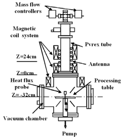
Figure 4. Experimental setup
