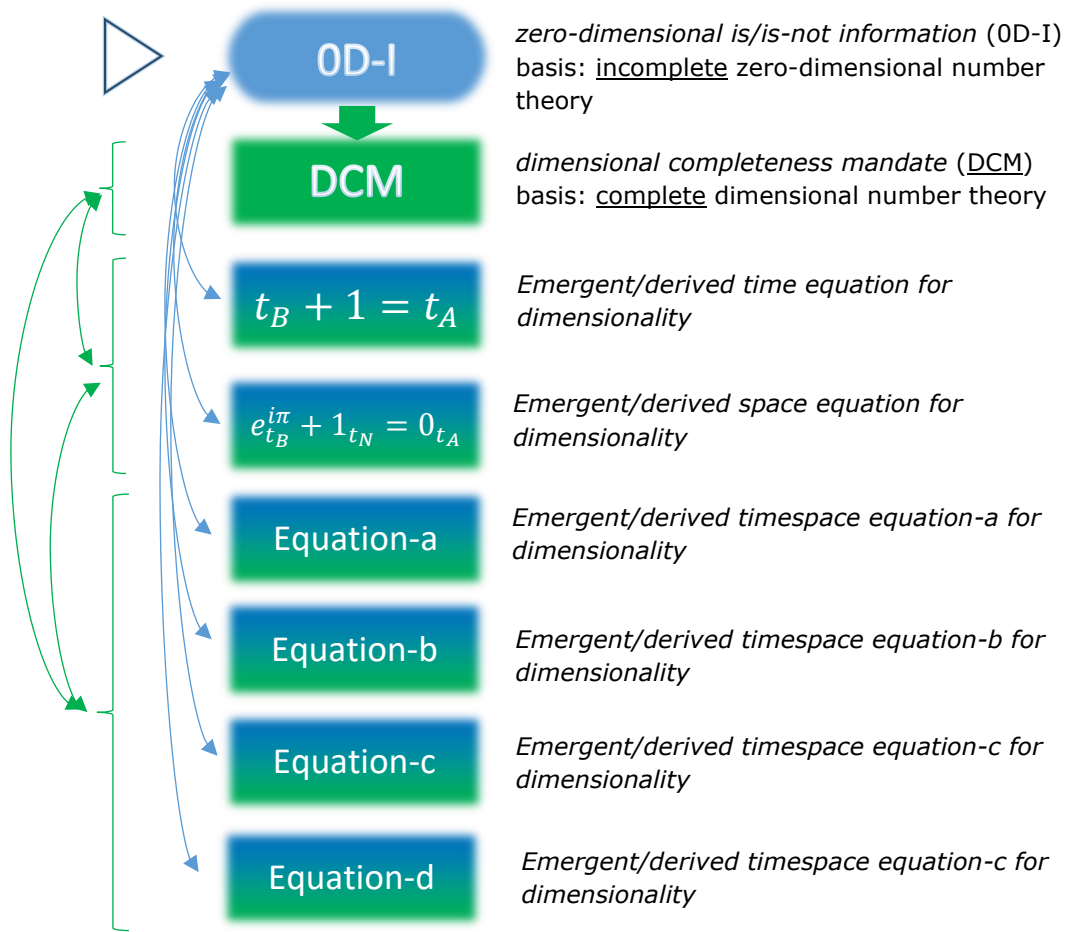
Figure 14: figure 4 as a top-down hierarchy of number theory regard, from the incomplete zero-dimensional number theory basis (OD-I) as the blue arrows/connectors, to then mandate the dimensionally complete number theory basis (DCM) as the green arrows/connectors.
