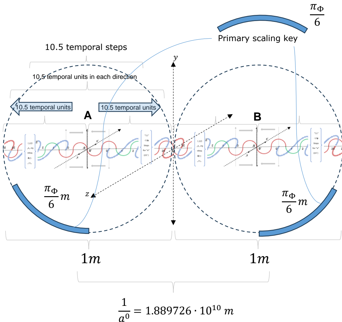
Figure 41: here \frac{\pi\Phi}{6} is the primary quantum wave function scaling key which when factored as a metric requires the Bohr radius a^0 to be factored into the resultant 1m diameter to test the proxy atomic radius analogue with the known atomic radius value a^0 , resulting in a new scaling value of 1.889726 \cdot 10^{10} m .
