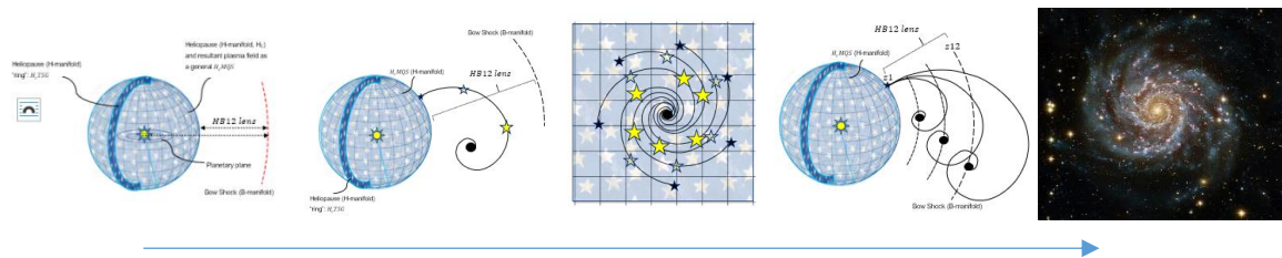
Figure 47: r_E TSG and associated HB12 scheme from paper 33 ([33]: p13-16, fig4-8).
