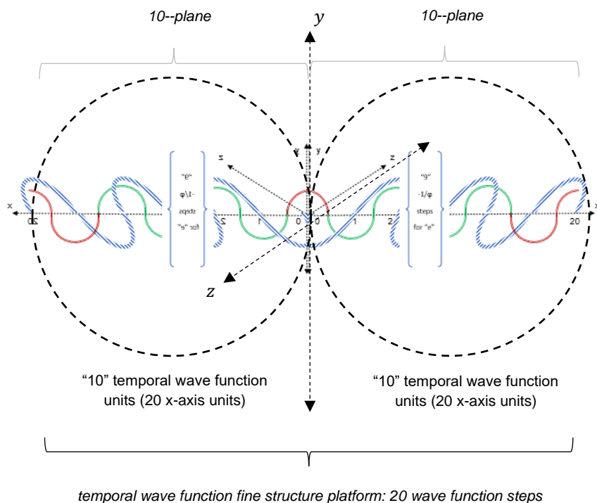
Figure 38: A temporal wave function 10-plane, namely “10” temporal wave function units as the basic temporal wave function scale in addressing the basic \pi -requirement of equation 10.
