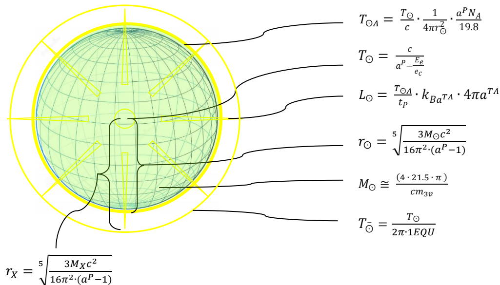
Figure 45: Highlighting the phenomenal features of Sol from the derived fine structure constant ( \alpha ) and Planck ( h ) values.
