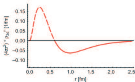
Fig. 1 Charge distribution in the neutron 1
