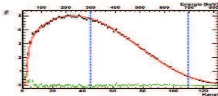
Fig.7 \beta -decay spectrum of the neutron (Ref 2)
