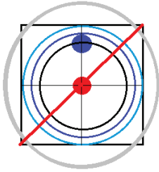
Fig. 2 Schematic two-dimensional representation of the neutron (not to scale)
