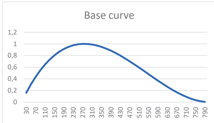
Fig. 6 Base curve: relative frequency (normalized to 1) of the energy terms (keV )
