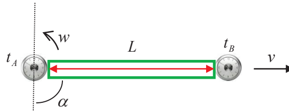
Figure 10: Rotating the Einstein's light clock.
