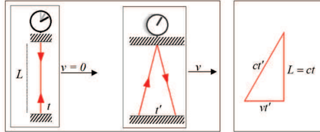
Figure 7: Einstein's light clock
