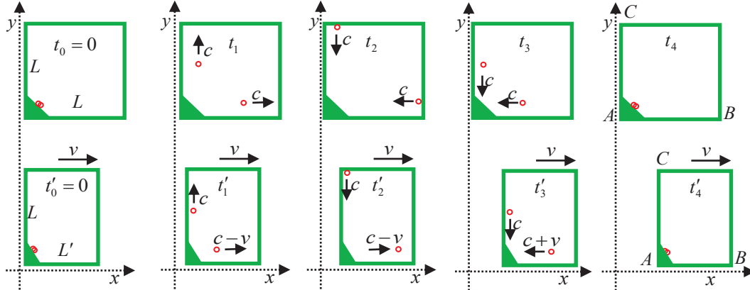
Figure 9 : Time frames for the rooms presented in Figure 8.
