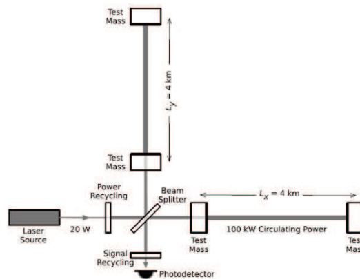
Figure 1: The LIGO detector: A modified Michelson interferometer.
