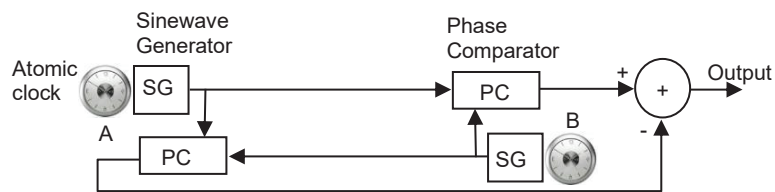
Figure 12: WUIT implementation using atomic clocks.
