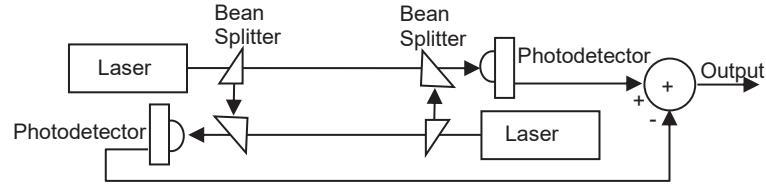
Figure 14: WUIT implementation using two Laser sources.
