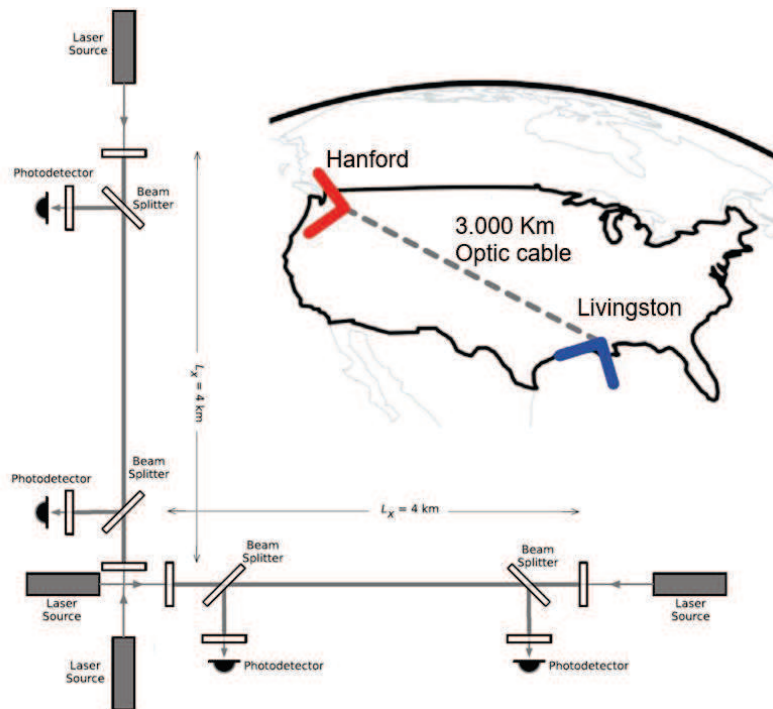
Figure 16: "Five-Arms" WUIT implementation integrated with LIGO detectors.
