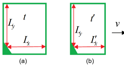
Figure 8: Two of Einstein's light clocks: a) room stationary; b) room moving at speed v .
