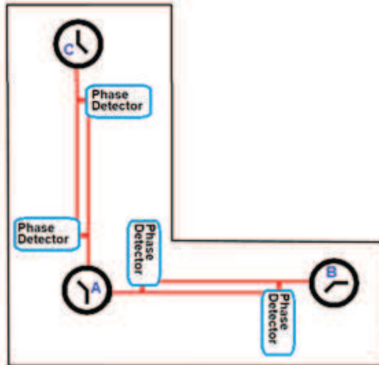
Figure 5: White-Ulianov Time Interferometer with two arms
