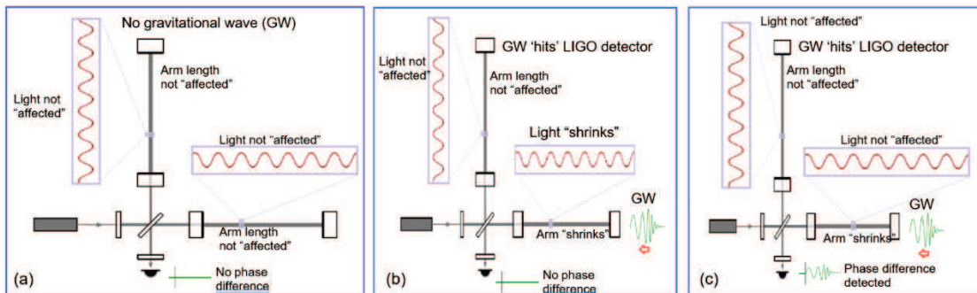
Figure 2: Three LIGO detector cases: a) No gravitational wave “hits” the detector. b) Gravitational wave “shrinks” the arm length and “shrinks” the light fields (no phase difference). c) Gravitational wave “shrinks” the arm length and light is not affected (phase difference detected).
