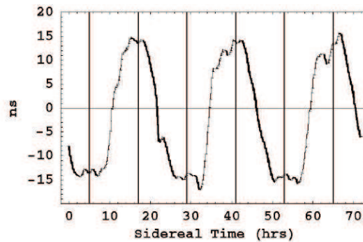
Figure 6: Phase drifts, as observed by Roland De Witte in 1991
