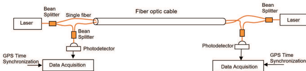
Figure 15: Implementation of WUIT using "all in fiber" optics.
