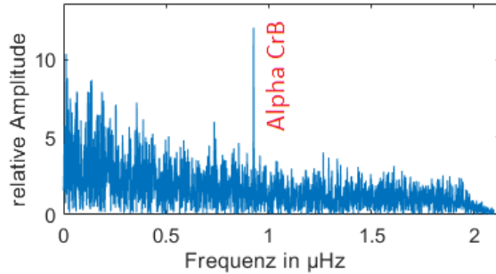
Figure 1): Spectrum of the GW of \alpha CrB after changing the frequency to f_{ZF} = 1/(300 \text{ hours}) and compensating the phase modulations. This increases the amplitude of the carrier frequency of the GW significantly. The vicinity of f_{ZF} is filled with the distorted spread spectra of previously undiscovered GWs of similar frequency.
