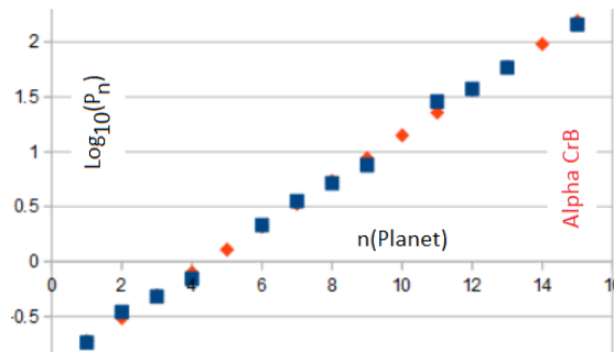
Figure 2): The logarithm of the orbital period of the planets (in years) of Alpha CrB as a function of their order. The actual values (blue) hardly differ from Dermott's law (red). Despite an intensive search, the PM of the "missing" planets could not be detected.
