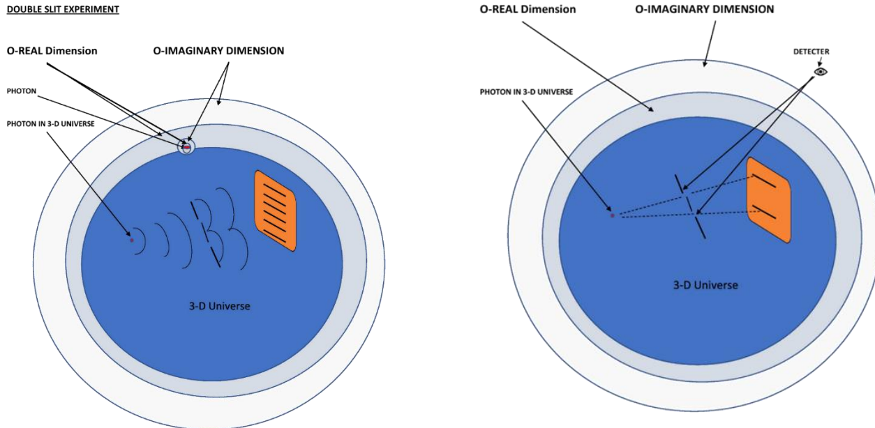
FIG 15: Unobserved travel of photons and observed travel of photons in a 3-D universe
