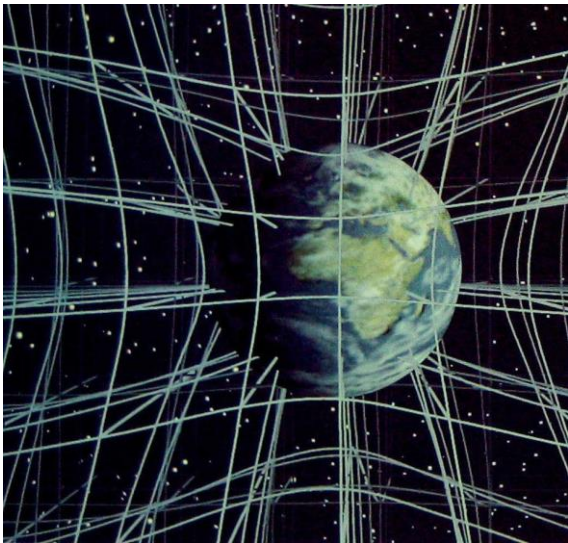
Fig 7: Picture of the energy line association with matter in a 3-D universe.
