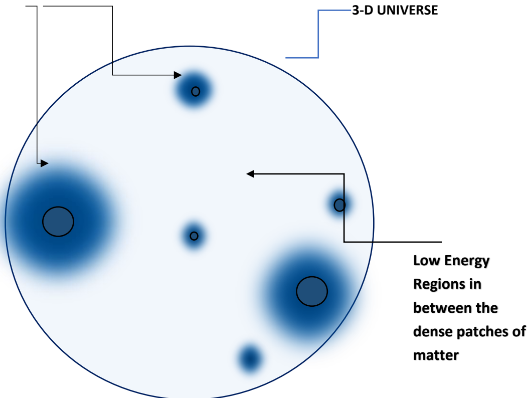
Fig 13: Low-energy regions in space give rise to the concept of dark matter.
