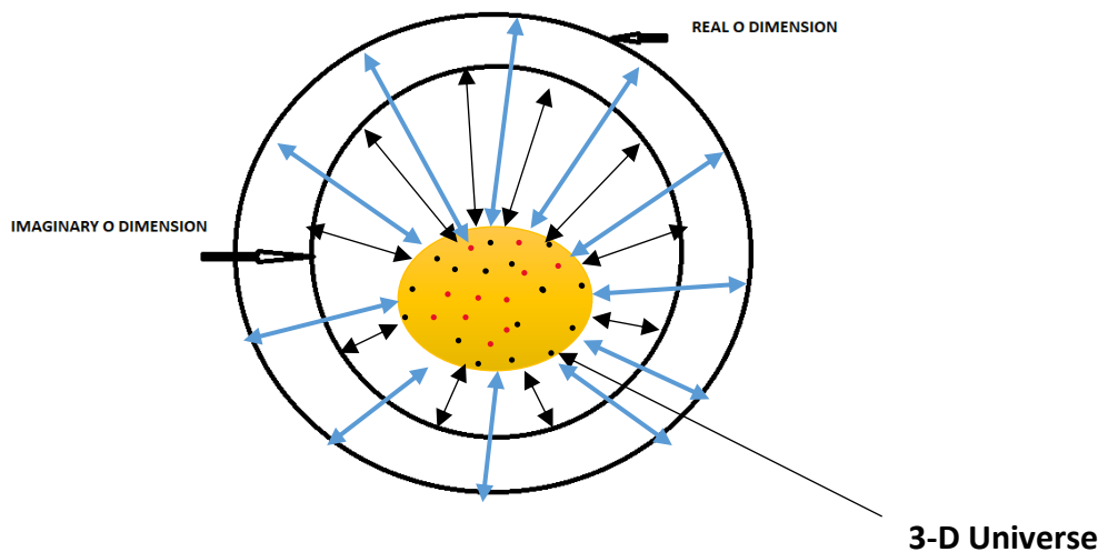
Fig 10: 3-D Universe vibrating between two 0-dimensions
