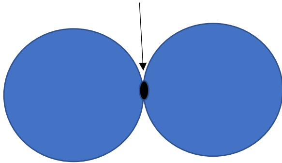
Fig 5: Beginning of the 3-D Universe, Time and Entropy
