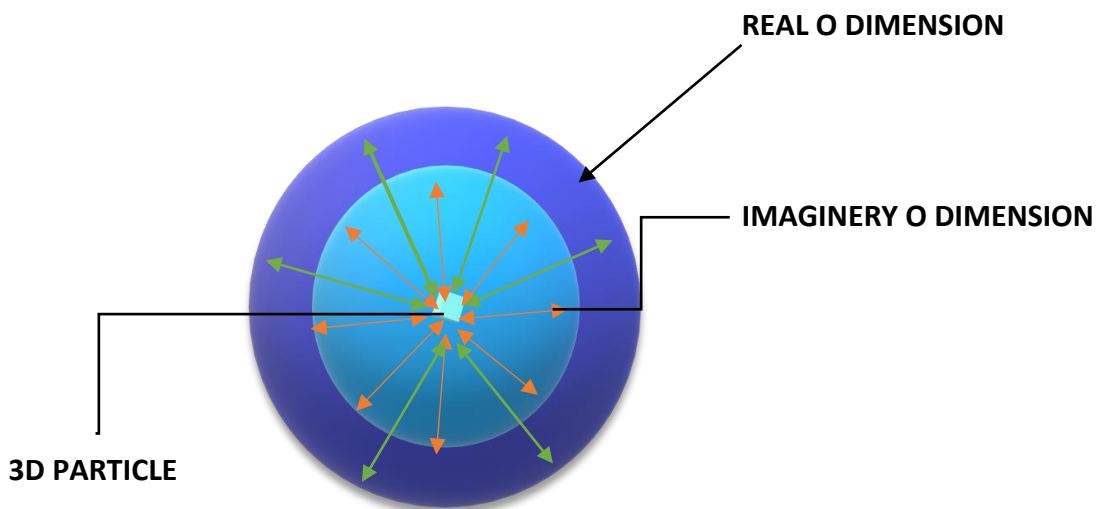
Fig 8: 3-D particle formed in between 2 O-Dimensions, a beginning of the 3-D universe
