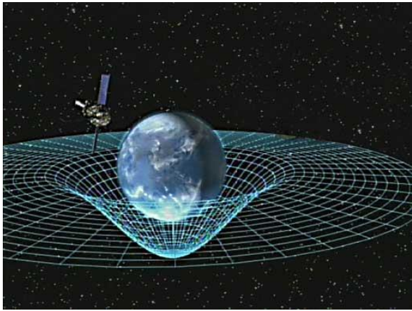
Fig 1: Space-time Curvature of General Relativity
