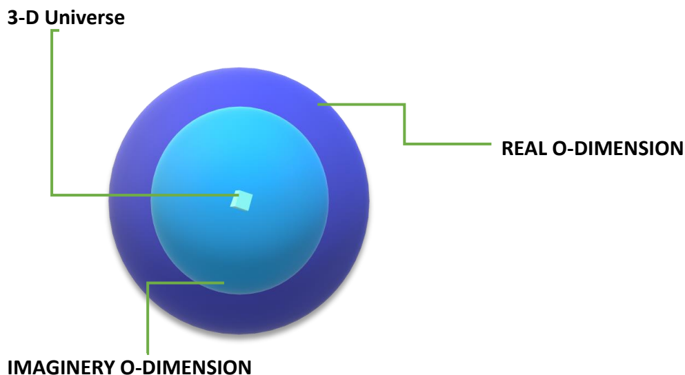
Fig 3: 3-DIMENSIONAL UNIVERSE AT THE CENTRE OF TWO O-DIMENSIONS
