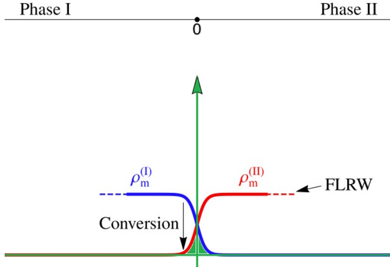
Figure 1: Transition from phase I to II in the universe proceeds by the conversion of matter made up from the degrees of freedom of frame (blue) to those of our T-dual frame (red). In our model the time t = 0 corresponds to energy scale \Lambda_{cr} . The small green area around t \sim 0 is the new second topological phase O, to be discussed in subsection 3.3. In the other topological model the point t = 0 is near Planck scale. In the SM t = 0 corresponds the GUT scale. (Figures 1, 2, and 4 are from [1] with permission.)
