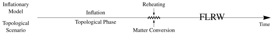
Figure 4: Comparison between the inflationary and topological paradigms for the early universe. The topological scenarios replaces the period of accelerated expansion by a topological phase to explain homogeneity, isotropy, flatness and near scale invariance. In both paradigms, the universe for t > 0 is well described by the standard Big Bang cosmology.
