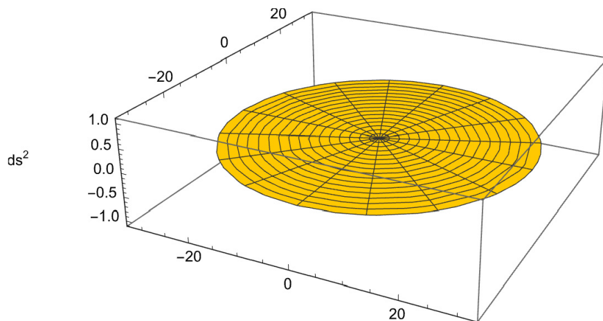
Figure 2: The figure shows the spacetime interval in the new metric as we move towards the center of the gravitational object. In this plot, we start at a distance of R = 30 \frac{GM}{c^2} and move inwards to R = \frac{GM}{c^2} .
