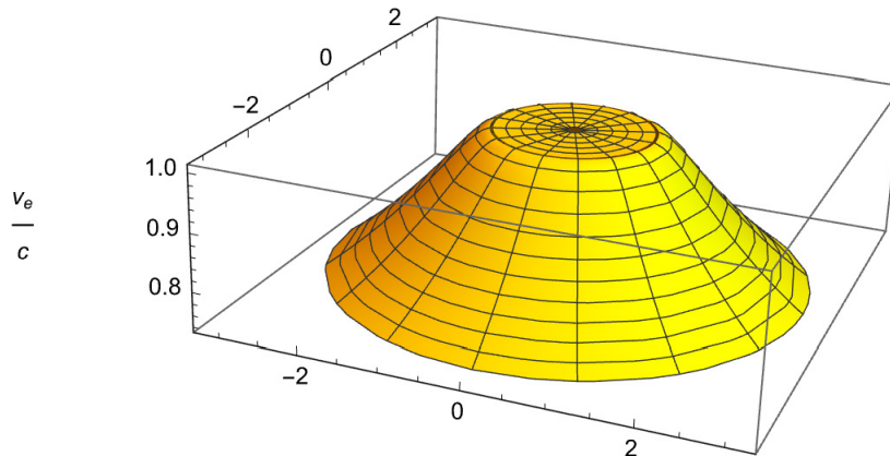
Figure 5: The figure illustrates the escape velocity from our new metric on the inside as well as on the outside of a black hole. The graph is starting at r = 3\frac{GM}{c^2} = 3r_c from the center of the black hole and down and including r = l_p . Be aware that the radius where the escape velocity is c is at \frac{GM}{c^2} and not at \frac{2GM}{c^2} as is predicted in the standard Schwarzschild metric. The vertical axis is \frac{v_e}{c} . As we can see is the escape velocity is never above c inside the black hole and always below c outside the hole.
