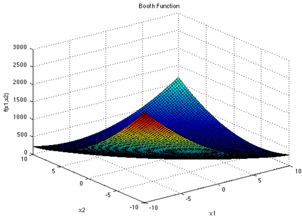
Figure 5. Booth Function
