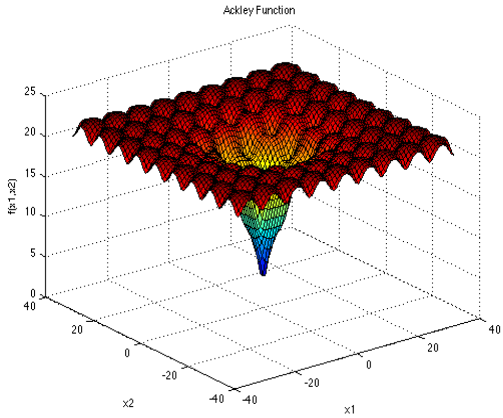
Figure 2. Ackley Function
