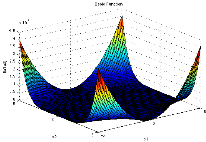
Figure 3. Beale Function
