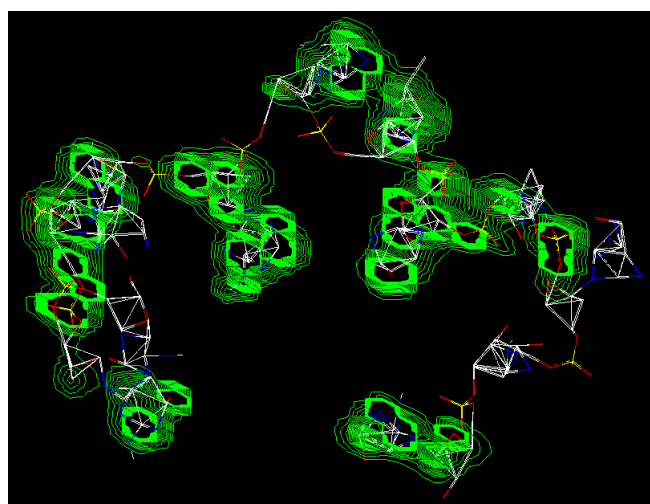
Figure 6: Image of [1bna]Si DNA macromolecule. The Figure represents a third structure obtained after molecular dynamics, for the [1bna]Si DNA molecule, in 2D contours of its electrostatic potential. Source: [Authors].
