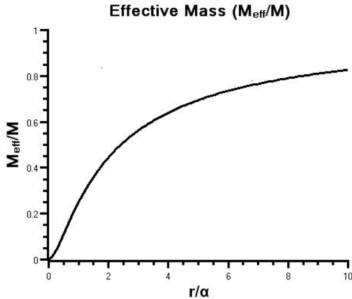
Figure 2: Effective gravitational mass
