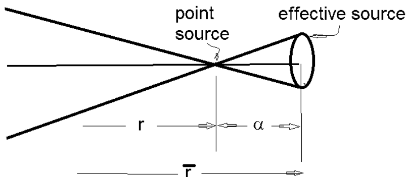
Figure 3: Due to angular curvature the point source appears as a ring
