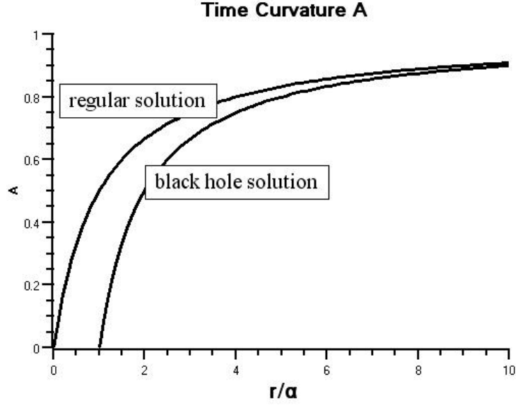
Figure 1: Time curvature A
