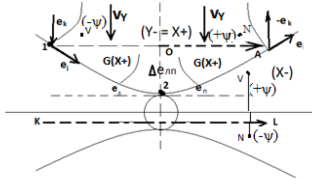
Fig. 6. Quantum gravity ( X + = Y- ) a mass field.
