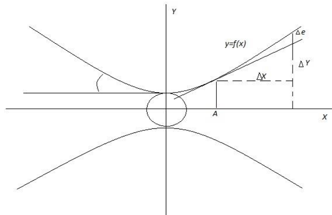
Fig.3. Quantum ( X \pm ) of dynamic space-matter.
