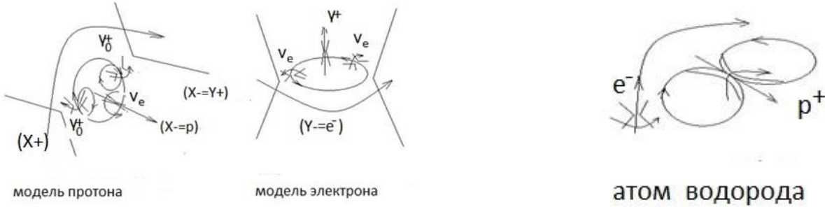
Fig.5. Mass fields of an atom.
