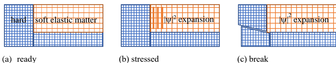
Fig.19 The nucleon density expansion continues until the stress has risen sufficiently to break through the resistance, suddenly allowing sliding over the locked portion of the fault, and releasing the stored energy.
