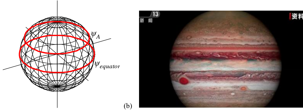
Fig.10 (a) Mutual cascade-interference will lead to the acceleration-roll wave having the same phase. (b) Jupiter (the photo from News).
