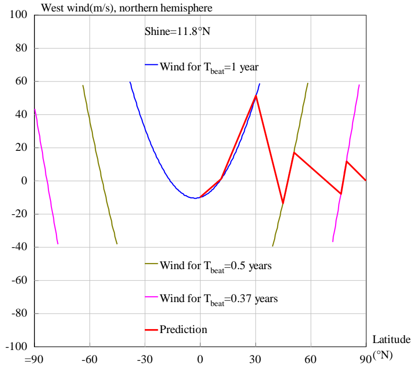
Fig.18 Japanese latitude is about A=30^\circ\text{N} , where Japan has almost the strongest mean wind at altitude 200hPa. <Clet2020 Script> [26] //see Fig.11(a)
