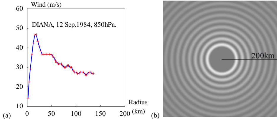
Fig.15 (a)Gradient wind as a function of the radius for the hurricane DIANA (12, Sep.1984) measured at 850hPa [40]. (b) The simulation of a cyclone using acceleration-roll wave, |x| < 200\text{km} .
