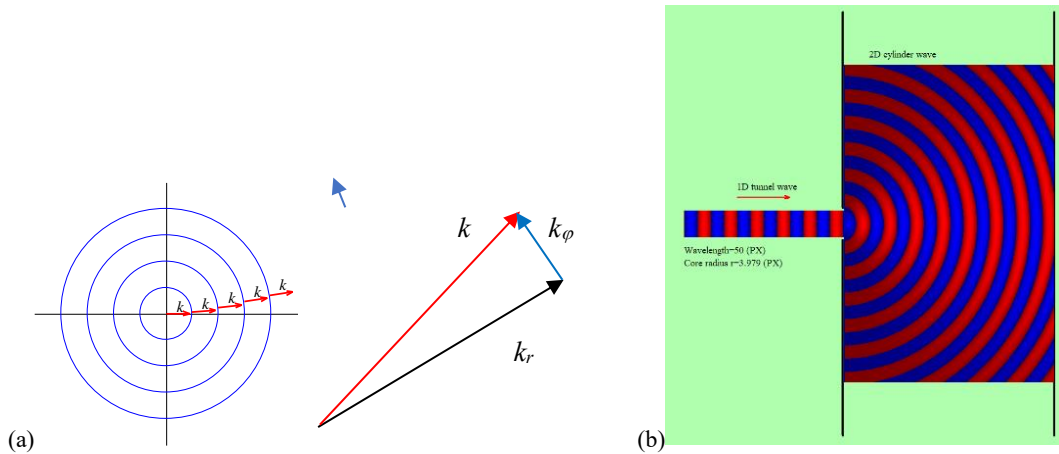
Fig.17 (a) 2D wave-vector \mathbf{k} spins little by little in the cylinder coordinates (r, \varphi) . (b) from 1D to 2D, the spin works to split the electron beam due to the double-value k_\varphi .
