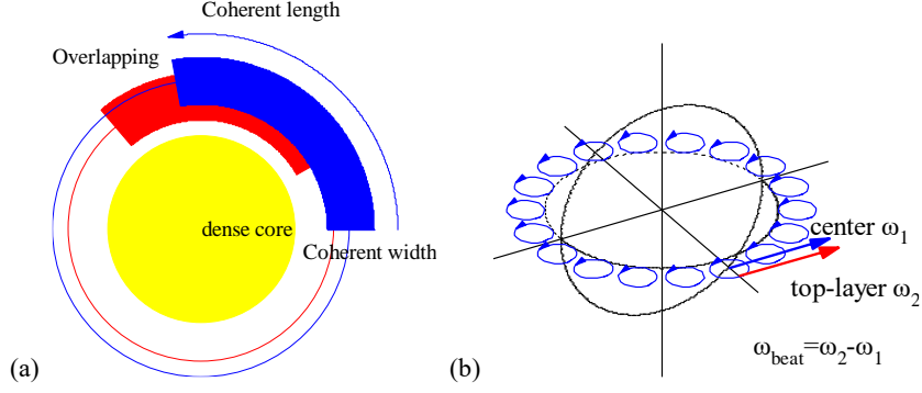
Fig.9 (a) Illustration of overlapping in the coherent width direction. (b) In convective rings at the equator, the speed difference causes a beat frequency.
