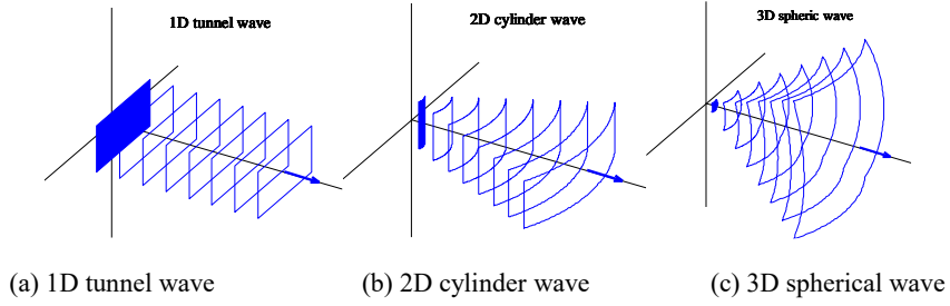
Fig.16 The wave behavior in various dimensional spaces.
