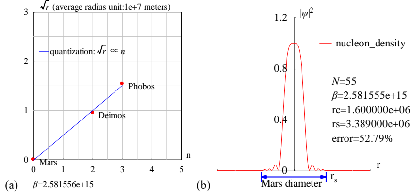
Fig.8 (a)Quantization of Mars and its satellites. (b)The matter distribution |\psi|^2 around Mars has been calculated in the radius direction.
