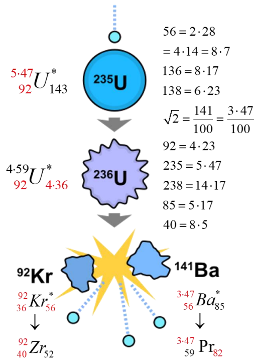
Stable numbers are marked in red Fission of U235 and its Explanations
