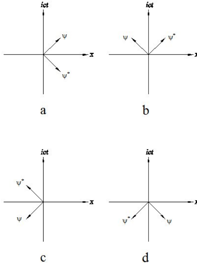
Fig. 2 four forms of \psi and conjugate state \psi^* ,
