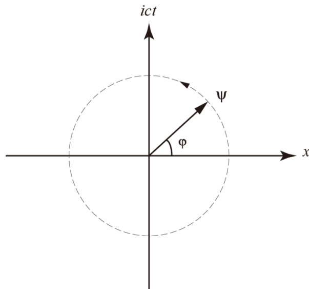
Fig. 1 Space-time wave representation of wave function
