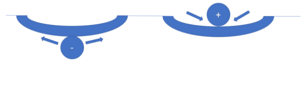
FIG. 2: Negative matter applies positive gravitational mass to positive masses and negative gravitational mass to negative masses.
