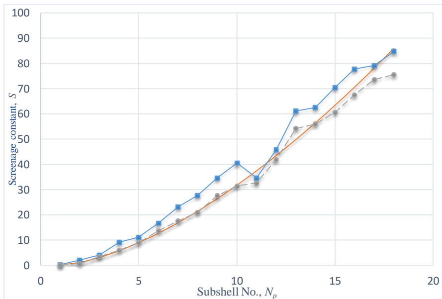
Fig. 3. Dependence of the constant of shielding S on the serial number of the subshell N_p . ● – in this article; ■ – acc. to Slater; red line – according to equation (4) at b=2/3
