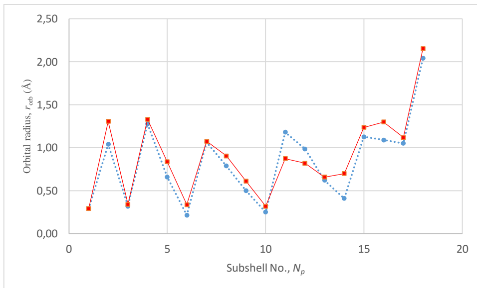
Fig. 5. Dependence of the orbital radius r_{orb} of an atom on the serial number of the closed subshell N_p : • – data from work [8], ■ – according to the equation (6).
