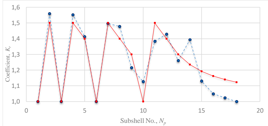
Fig. 4. Dependence of the coefficient K_r on the sequential number of the subshell N_p : • – calculated data, ■ – according to equation (5)
