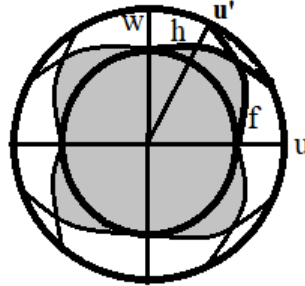
Figure 1. u - w plane, where the radius of the smaller circle is 0.700001,
