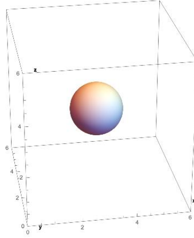
Figure 1: The figure shows one indivisible particle. If it is at rest, it is a scalar. However, indivisible particles when not colliding are energy that moves at speed c (velocity \mathbf{c} ). Since the motion is in a direction, they are vectors.
