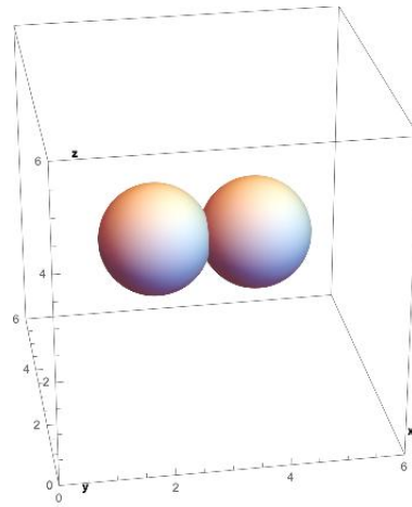
Figure 2: The figure shows two indivisible particles colliding; this structure is what we call mass, and it can be simplified by being described as a vector, as the two-sphere structure has direction in space.
