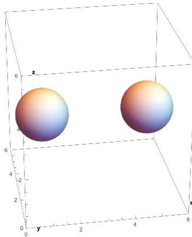
Figure 3: The figure shows two indivisible particles traveling after each other with a distance from center to center equal to the Compton wave. This is a vector.
