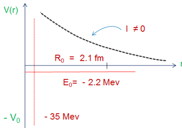
Figure 1. Plot of Effective Square-well potential.
