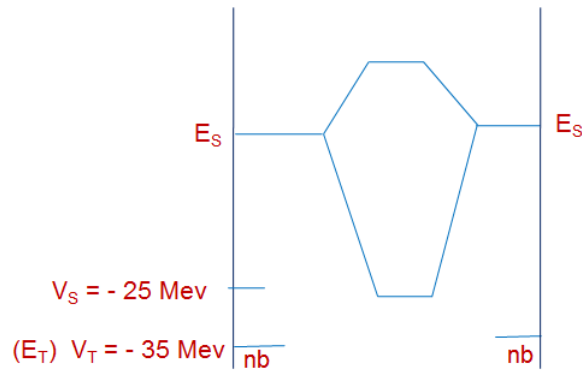
Figure 2. Energy Level Diagram showing bonding of excited level state in comparison to non-bonding ground state of deuteron.
