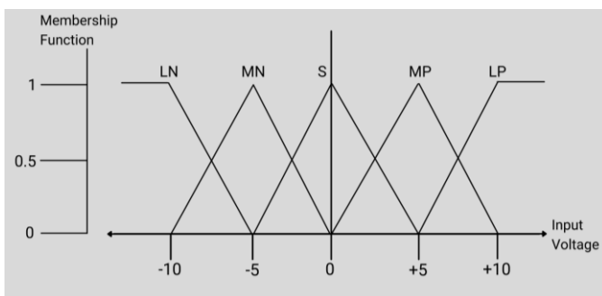
Figure 7: Membership Functions for LP, MP, S, MN and LN.
