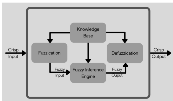
Figure 4: Fuzzy Inference System
