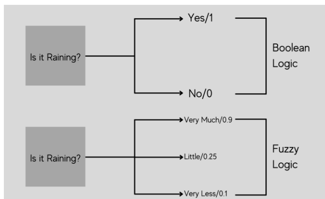
Figure 1: Fuzzy Logic
