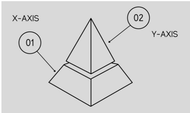
Figure 6: Membership Function
