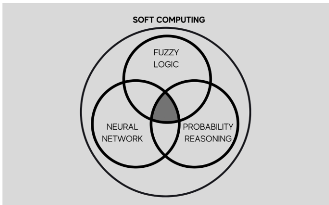
Figure 3: Soft Computing
