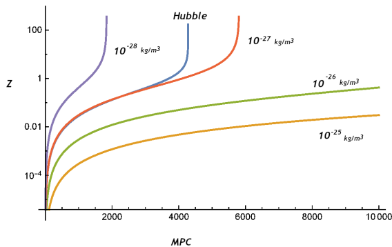
Figure 1 The trace labeled Hubble was computed using equation 11 with H_o = 70 \text{ km/secMPC} where 1 \text{ MPC} = 3.262 \times 10^6 \text{ light years} = 3.086 \times 10^{22} \text{ meters} for an expanding universe. All the other graphs were computed from equation 10 for photon propagation. What is interesting is the Hubble result almost falls on the line at lower z values for a mean density of 10^{-27} \text{ kg/m}^3 . The graphs represent difference between massless fields against the acceleration of a massive particle's proposed behavior. The dark energy was a result of the split between the density based response at 10^{-27} \text{ kg/m}^3 verses the Hubble computed response and shows the data was fitted to the wrong model. The net result is that there is no dark energy.
