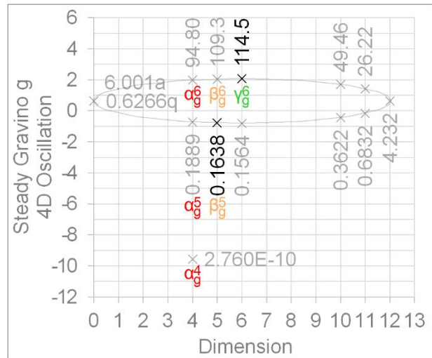
Fig. 5 The oscillating masses of gravinos
