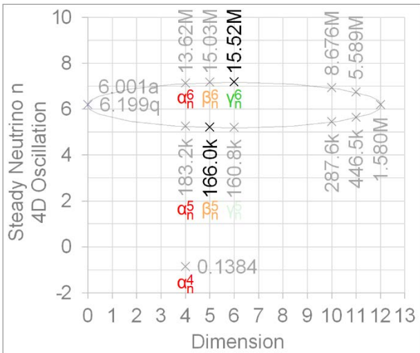
Fig. 4 The oscillating masses of neutrinos
