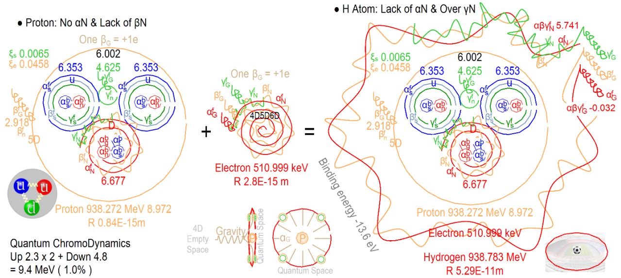
Fig. 1 Shape of proton, electron, and hydrogen
