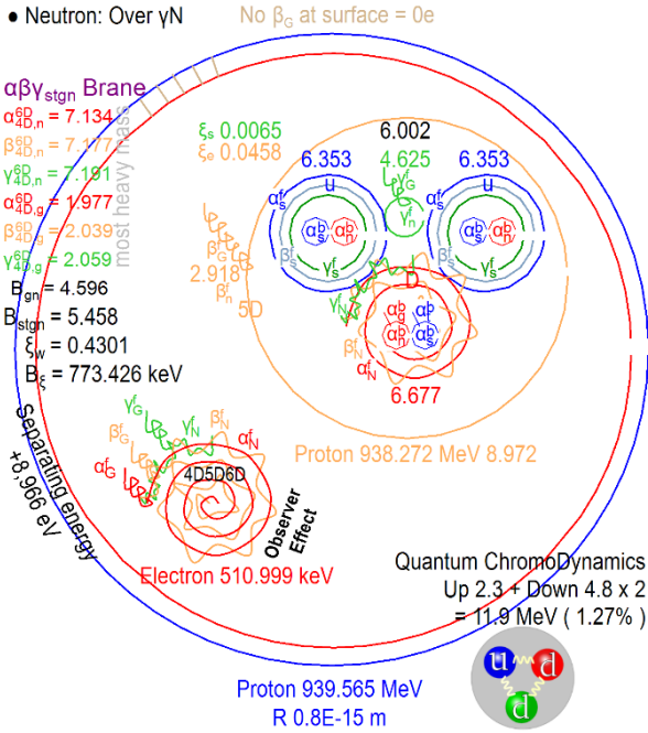
Fig. 3 Shape of neutron
