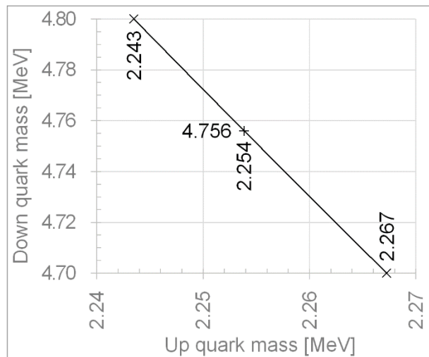
Fig. 2 Relation of up quark and down quark masses
