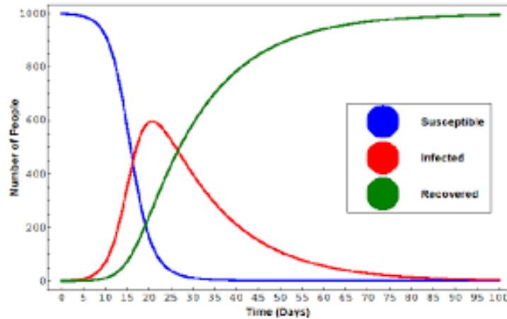
Figure 1. Schematically depicted SIR model with three compartments
