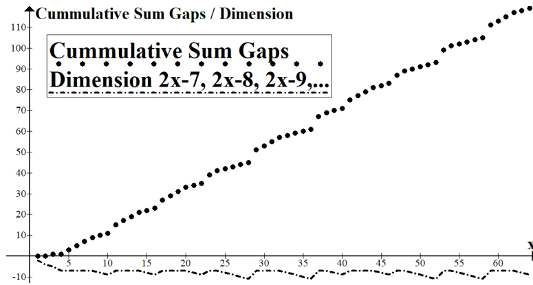
Figure 11. Prime-Composite finite scale mathematical (graphed) landscape. Data for x = 2 to 64
