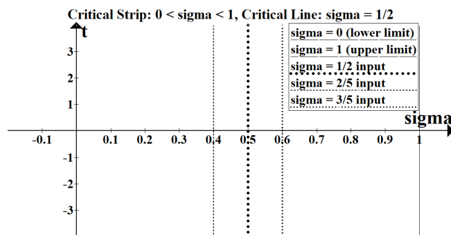
Figure 7. INPUT for \sigma = \frac{1}{2}, \frac{2}{5}, and \frac{3}{5} . \zeta(s) has countable infinite set (CIS) of Completely Predictable trivial zeros at \sigma = all negative even numbers and [proposed] CIS of Incompletely Predictable nontrivial zeros at \sigma = \frac{1}{2} for various t values.
