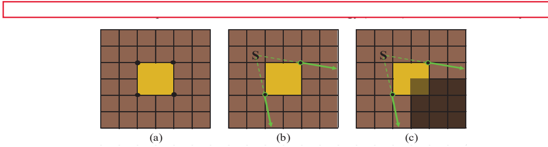
Figure 4. (a) A rectangle with its four vertices highlighted. (b) The two relevant points and casted rays for this rectangle. (c) The cells occluded by the rectangle are darkened.
