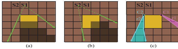
Figure 6. (a) Rays and cell visibility for S1. (b) Rays and cell visibility for S2. (c) The rays pairs forming two cones C1 and C2, with their origin points marked with a circle. The rays forming C1 are cast from the same point, while the rays forming C2 are cast from different points.
