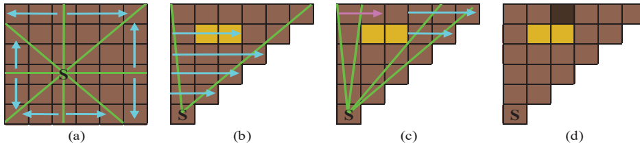
Figure 2. (a) An FOV grid split into octants with row/column traversal shown. (b) Traversal of an octant until vision-blocking cells are encountered. (c) Traversal of a sub-octant after the traversal is split by the vision-blocking cells. (d) The resulting FOV.
