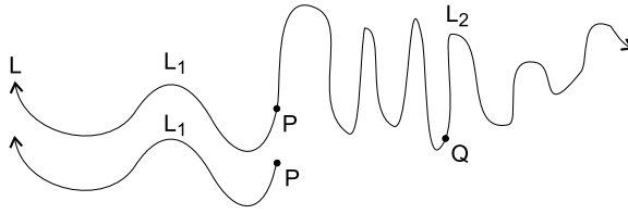
Figure 16.6 – In the Euclidean space all lines* have a finite length.
