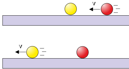
Figure 32.1 – Elastic collision of two particles: the linear momentum and the kinetic energy are preserved (in the case represented the two particles have the same mass).
