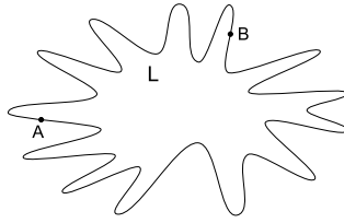
Figure 16.3 – All closed lines* have a finite length in the Euclidean space.
