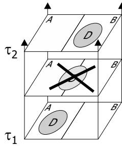
Figura A.3 – In the discrete spacetime of a CALM, an object D changes from A to B without passing between A and B (think, for instance in a quantum jump of an electron).
