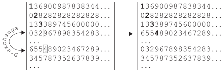
Figure 11.1 – The fourth row of T before being d -exchanged (Left); and after having been d -exchanged (right). Note that only the digits of the decimal expansions are represented, not including the initial 0 or the subsequent decimal separator.
