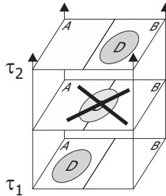
Figure A.3 – In the discrete spacetime of a CALM, an object D changes from A to B without passing between A and B (think, for instance in a quantum jump of an electron).
