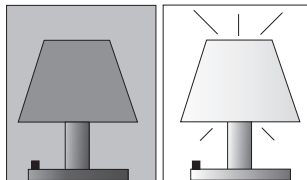
Figura 23.2 – Thomson's lamp has two, and only two, states: off and on . The state of Thomson's lamp changes if, and only if, its button is pressed.
