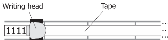
Figure 31.1 – The unary writing machine on the point of writing the fifth numeral, i.e. the number 5 in the unary numeral system.
