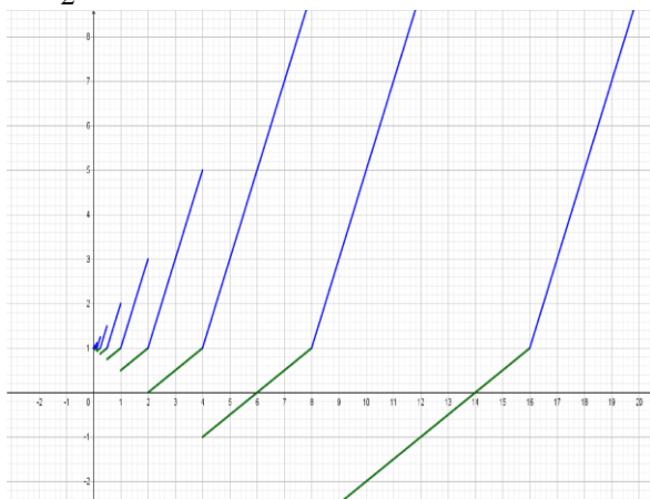
Figure 1. The graph of K_2 and K_{1/2}
