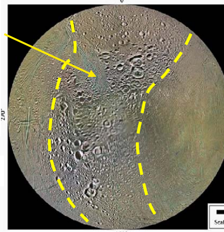
Northern Hemisphere
