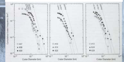
Fig. 12. Isochrones and crater-size frequency measurements for nine debris aprons in Tempe Terra. Numbers in the boxes refer to the names labelled in Figure 2. Segmented and stair-stepped curves indicate multiple resurfacing events, and shallow segments suggest the continuation of denudation and/or resurfacing. Absolute ages are in the range of few tens of Ma, with early traces dating back to 100 Ma and up to 200 Ma ago. For all aprons, intensive thermochronological degradation with numerous subconcentric pits on the debris aprons complicates the derivation of proper ages so that these values are considered as absolute minimums. For the statistics see Table 4.
