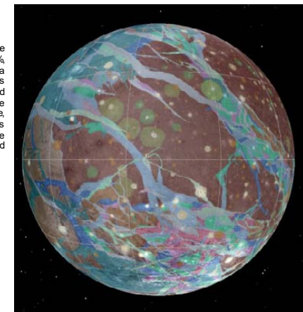
Satellite Image
