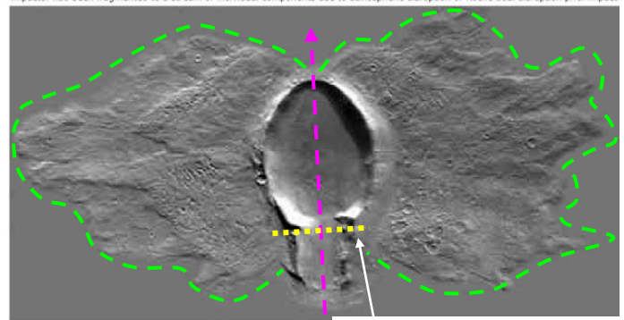
Example Mars Impact with Butterfly Ejecta distribution Credit: NASA / JPL / ASU / mosaic by Emily Lakdawalla Owing to the atmospheric drag, a string of fragmented impactors would differentiate during descent, with the larger bodies tending to travel further than smaller ones. We call special attention to the work of Schultz and Stickle ( Lost Impacts ), which explains how shallow angle of incidence (oblique) impacts generate "impact" structures that are significantly different from the classic, better understood, crater planforms. We proposed the Saginaw impacts to have been at an angle of less than 5 degrees - nearly tangential. The craters generated would manifest
