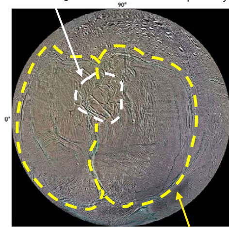
Trailing Hemisphere
