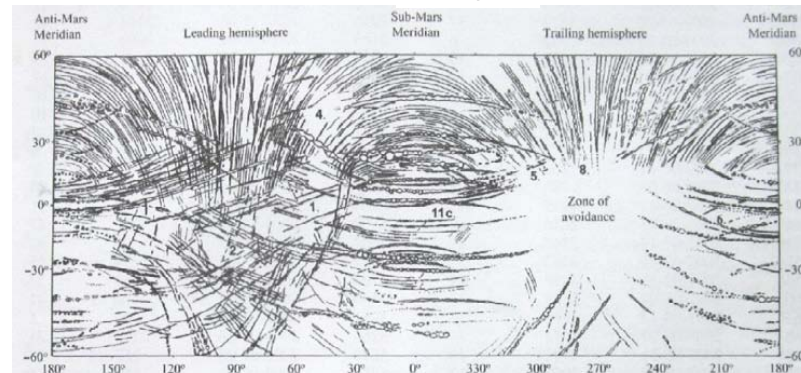
Fig. 1. Sketch map of grooves on the surface of Phobos derived from HRSC Mars Express , Viking and MGS ( Mars Global Surveyor ) images. A Mercator projection between -60° and +60° is used, and locations and orientations of features were assembled using crater positions from an existing control network (Duxbury & Callahan 1989). (1) Marks the centre of Stickney crater, the largest on Phobos; other numbers (2, 4, 5, 8 and 11c) refer to the approximate centres of figures in the text. Note that grooves become parallel along the sub-Mars and anti-Mars meridians (0° and 180°), and that there is a 'zone of avoidance' around which all grooves fade out and disappear surrounding the trailing apex (0° latitude, 270° longitude). The leading apex (0° latitude, 90° longitude) is characterized by groove families crossing each other at all orientations. from Page 24
