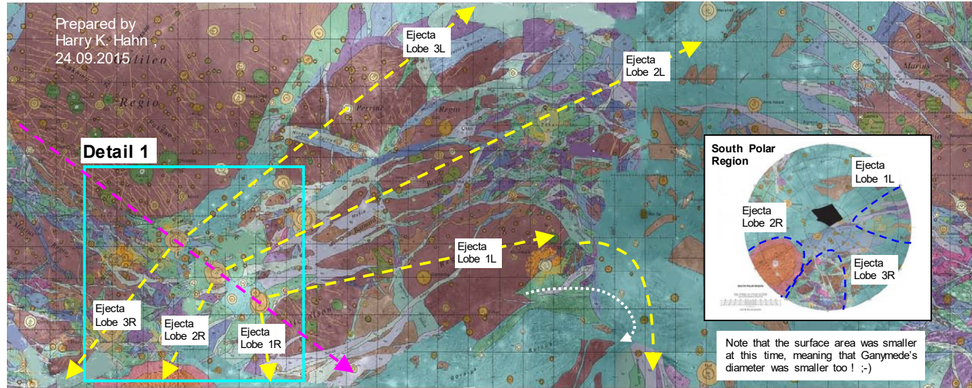
Image 1 : Manipulated Geological Map, showing roughly how the impact scene looked many million years in the past
