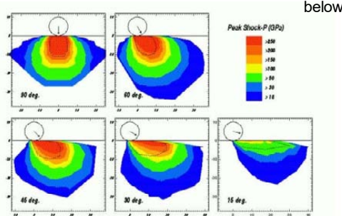
In the range of shock pressures at which most materials of geologic interest melt or begin to vaporize, we find that the volume of impact melt decreases by at most 20% for impacts from 90° down to 15°. Below 15°, however, the amount of melt in the target decreases rapidly with impact angle. Compared to the vertical case, the reduction in volume of melt is about 50% for impacts at 30° and more than 90% for a 15° impact. These estimates do not include possible melting due to shear heating, which can contribute to the amount of melt production especially in very oblique impacts.
