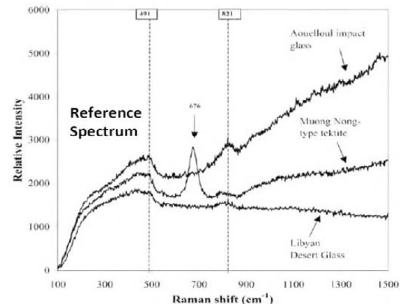
Fig. 8. Raman spectra of Anouelloul impact glass (a), Muong Nong-type tektite (b), and Libyan desert glass (c) generally exhibit two broad bands at 491 and 821 cm -1 and relatively high background fluorescence, which indicate a high degree of amorphization. These broad bands might be due to diaplectic glass. The numbers denote peak positions in cm -1 .
