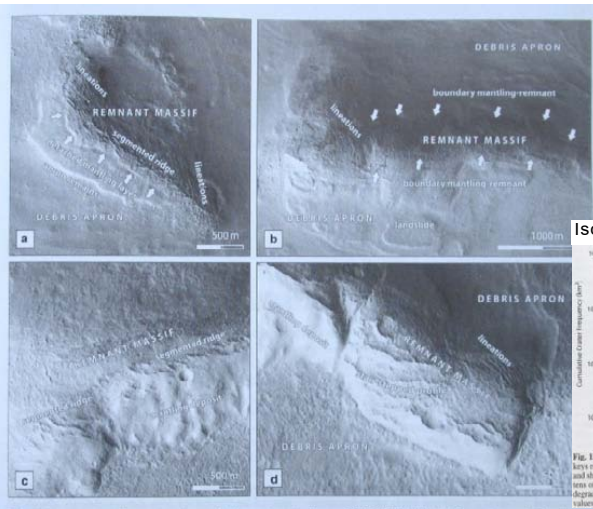
Fig. 6. Remnant massif constructs located in the western study area (278.5°E/49.5°N). (a) Remnant massif showing a dissected remnant surface in the detached mantling layer. The relict ridge at the crest indicates the former extent of the mantling material (CTX P19_008537_2285_XL48N080W, complex feature #41, Fig. 2). (b) Remnant massif with a detached mantling layer, which is partly draped over the remnant wall rock (CTX P19_008537_2285_XL48N080W, complex feature #41, Fig. 2). (c) and (d) remnant wall rock dissected by deeply incised gully features and stair-stepped profiles indicative of differential downslope mass movement and heavy degradation as suggested by impact-crater obliteration. Traces of remnant mantling layers are indicated at the footslope and remnant ridges on the wall rock (CTX P18_008102_2285_XL48N081W, feature #39, Fig. 2). North is up in all images. Image credit: NASA/JPL/MSSS.
