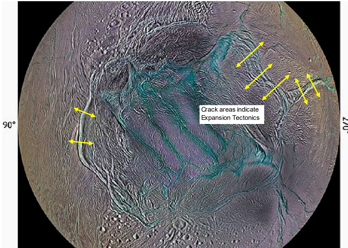
Detail view of the Tiger Strips area on Enceladus Southern Hemisphere
