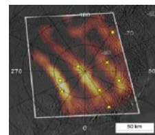
Enceladus heat color map
