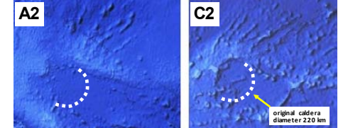
These two different ocean floor areas A2 & C2 which are thousands of km apart represent the same structure !! These "drift-off-copies" are an image of the first magma eruption which took place on position A1 ! These nearly identical structures, from two different crust layers (?), probably show the remains of a burst shield-volcano with a base Ø-450 km and a caldera Ø-220 km.
