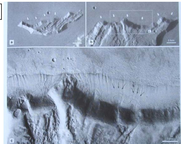
Fig. 10. Lobate debris aprons at isolated remnants in western Tempe Terra. The distribution and dimensions of lobate debris aprons in this more southern part are different from features located in more northern locations of Tempe Terra (Fig. 11). (a) Massif at 35.36°N with lobate debris aprons (white arrows) on the northern side, but not on the southern side (detail of HRSC image h5081_0000; centre at 35.36°N and 268.65°E; north is up, illumination is from the west/left). (b) Remnant highland massif with marginal lobate debris apron (white arrows). Lineations on lobate debris aprons are parallel to the inferred flow direction (detail of HRSC image h5081_0000; centre at 35.0°N and 267.9°E; north is up, illumination is from the west/left). (c) Detailed view of lobate debris apron shown in (b); a convoluted or undulating pattern in plan view characterizes the texture of the upper (southern) parts of the apron. The position of lobes (e.g. black arrows) are controlled by indentations of the southern scarp (detail of CTX image P17_007852_2154; north is up, illumination from the SW/lower left). Image credit: ESA/DLR/FUB and NASA/JPL/MSSS.
