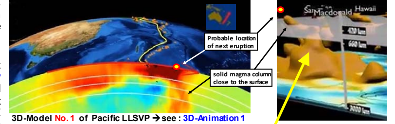
The Pacific-ULVZ is orientated along the path of a main ejecta ray of the PT-I
