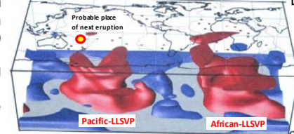
A 3-D view of the Pacific- & African LLSVP and the probable location of the next eruption
