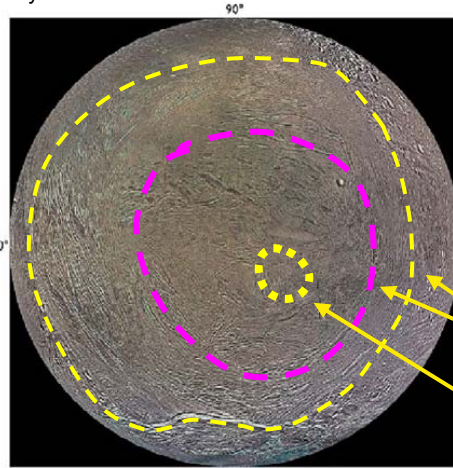
Leading Hemisphere
