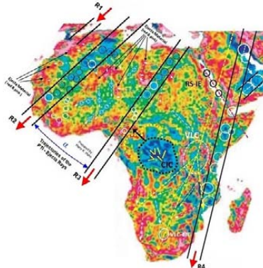
Gravity Anomaly Map of Africa showing the PTI-Ejecta Rays R1-R4
