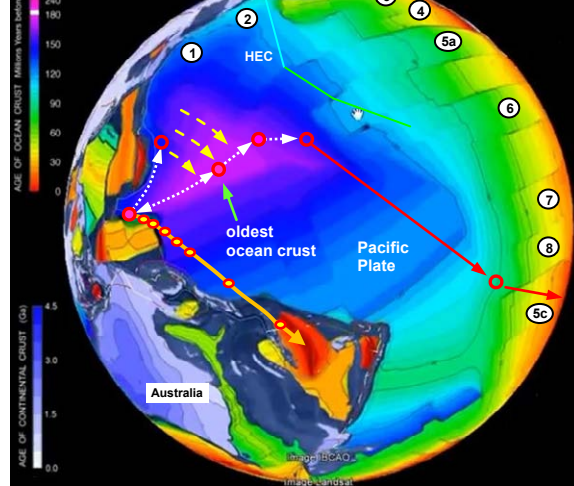
Ocean Crust Age Map :
