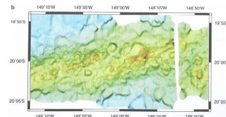
Fig. 1.12. a Bathymetry of a segment of the Vōa Tau Phi Ridges near Tahiti (Clouard et al. 2003). These volcanic ridges are clearly constructed by the superposition of many small, flat-topped volcanic cones. The Simrad EM12D, Hydrosweep DS and Seabeam multibeam bathymetry is shown using a 100 m grid interval and shading by slope magnitude. b Detail of volcanic morphology of ridges in region shown by box in a
