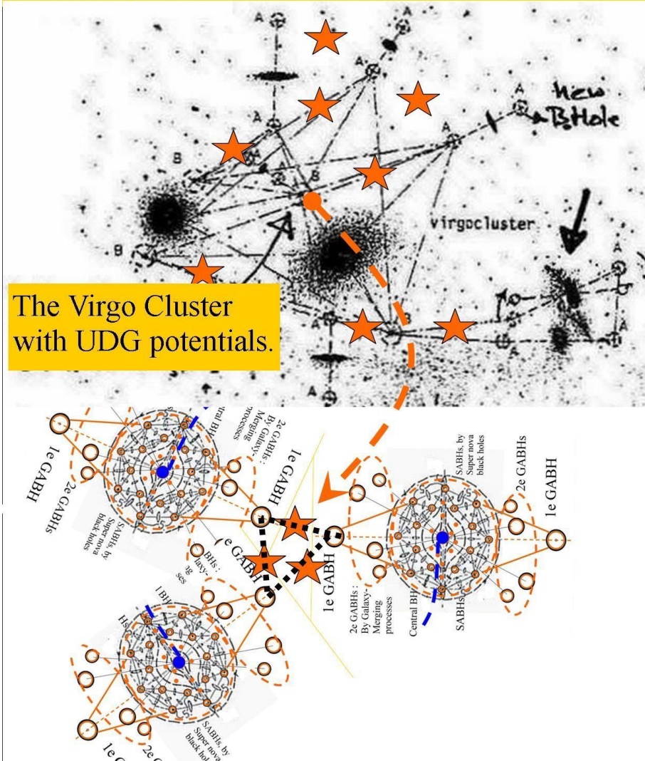
Figure 24. How galaxy clusters come together, with faint new formed galaxies in the center.
