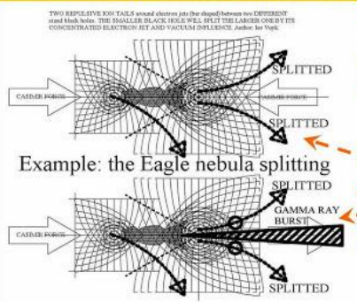
Figure 31, Black Hole Ratios with absorbing consequences.
