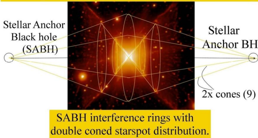
Figure 9, The Red Square Planetary nebula MWC922, equipped with double cone structure of expelled material including trailing starspots (Micro Black Holes). There are FOUR cones of interferences originated by the two Stellar Anchor black holes (SABHs). These four cones seem to interfere with the TWO cones of expelled material of the star, leading to FOUR rings of interference.
