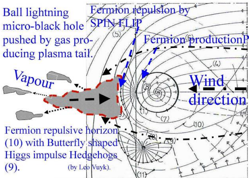
Figure 35., Details of vacuum synchrotron motion around a black hole with plasma creation and tail.
