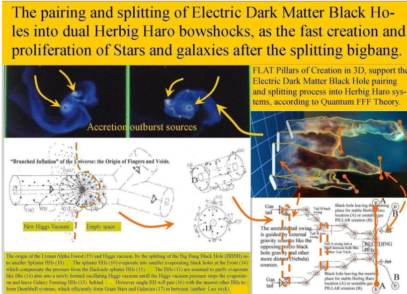
Figure 18, Examples of HH objects and dual DMBH pairing
