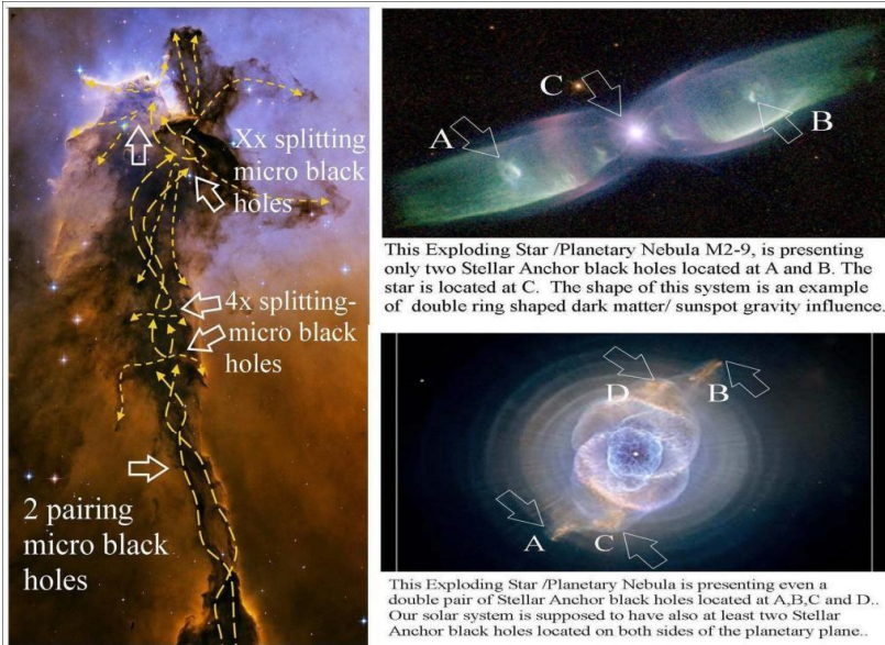
Figure 12, The Spire Eagle nebula, with two Planetary nebula, examples of the importance of black holes in the universe.
