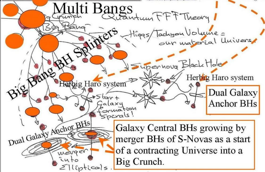
Figure 25, The big Bang splitting of the Dark Matter Black Hole nucleus.
