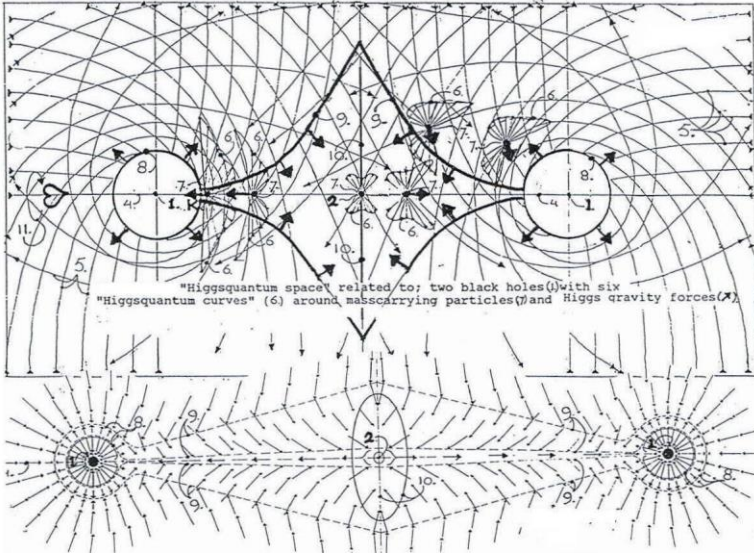
Figure 10, Axion Higgs Vacuum structure around a set of two Black holes, as is found to be present around Planetary nebula and early Galaxies and Herbig Haro objects.
