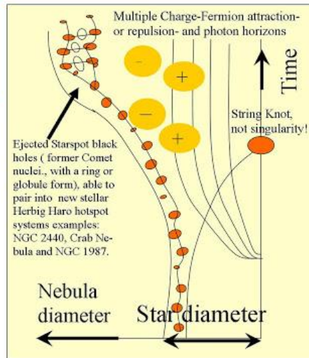
Figure 30, Super Nova Starspot Black Holes forming small Herbig Haro systems.
