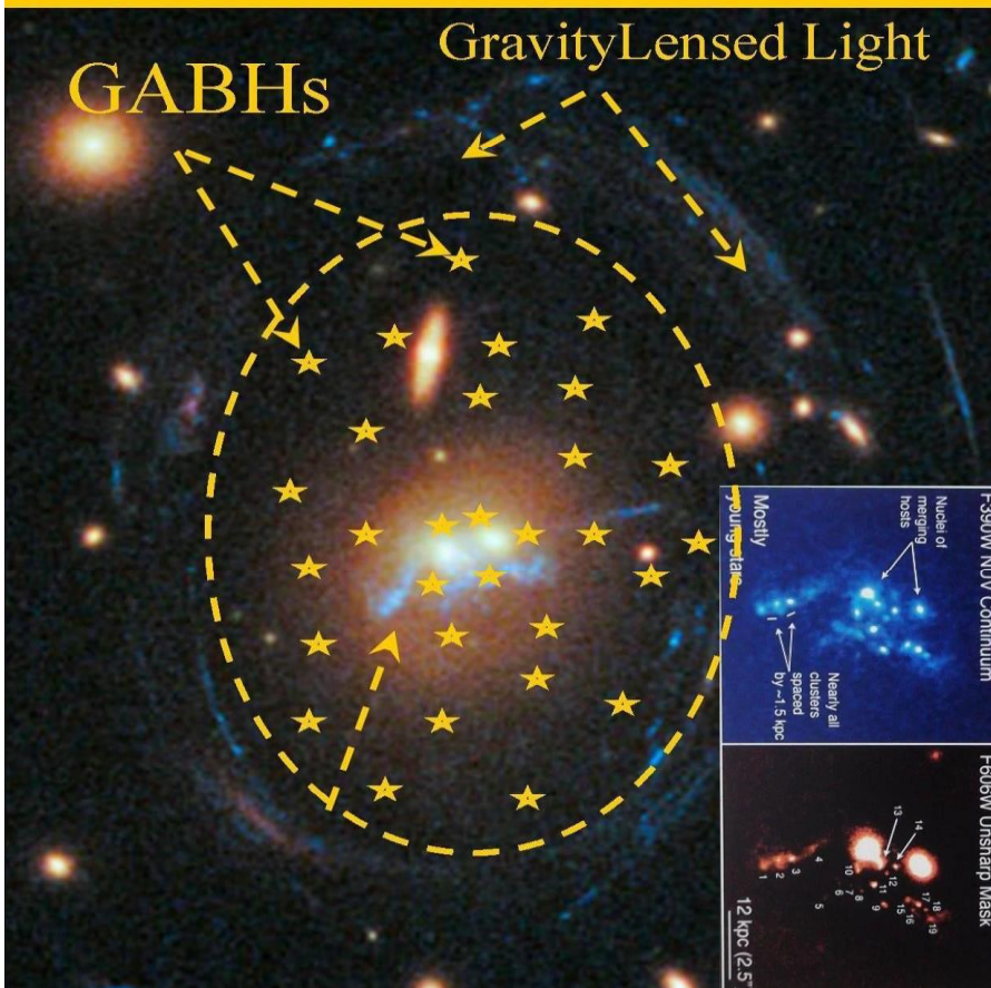
Figure: 16, Gravity lensed light through central hole in the globular Shell of Dark matter Black Holes or Galaxy Anchor Black Holes ( GABHs). The absence of GABHs in the centre is supposed to do the job.
