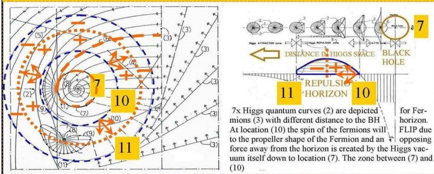
Figure 14, Principle of Fermion repulsion around a black hole according to Quantum FFF theory..
