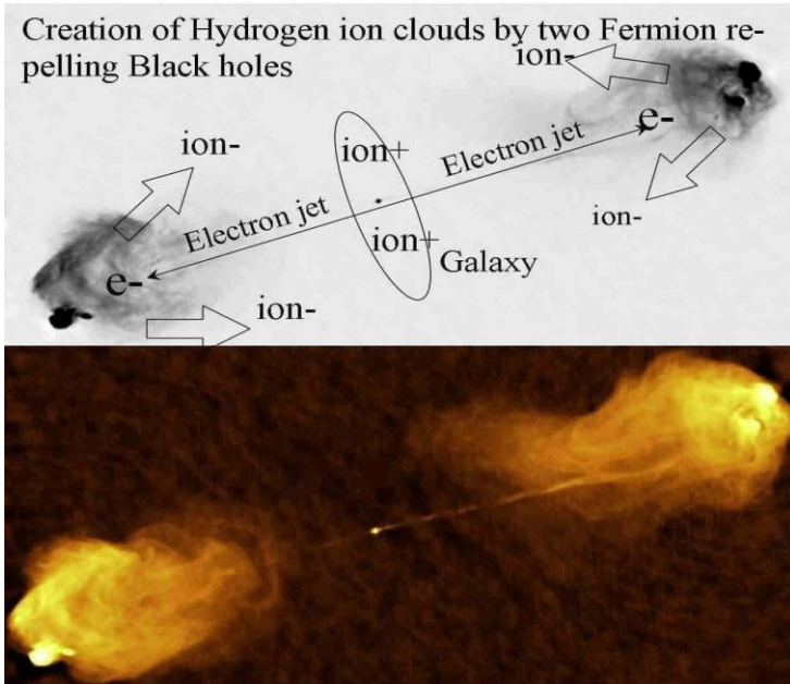
Figure 11, Cygnus A, equipped with Galaxy Anchor Black Holes (GABHs) clear electron jets and Hotspots, showing ionized gas production.
