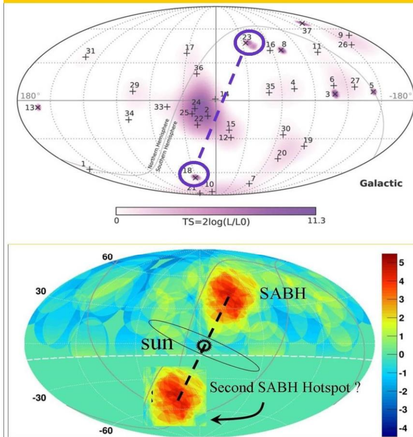
Figure: 15, Dual Stellar Anchor Black Holes around the earth !!
