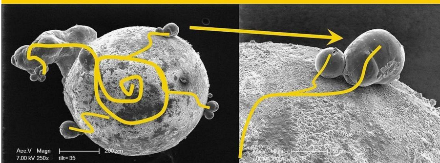
Figure 29. Magnetic Interference microscopic Higgs black holes, ( quantum Knots) with heating effects in silicon and as CERN LHC UFO dust particles.
