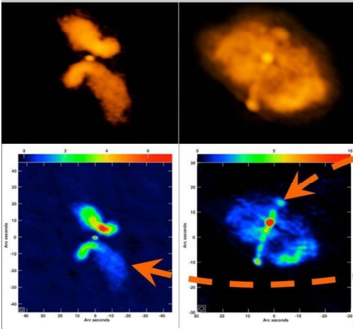
Figure 19, Abundance of X shaped radio sources.
