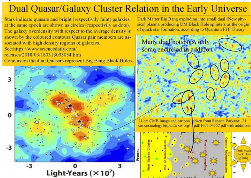
Figure 13, Dual Quasar/ Galaxy and Cluster forming relation in the early universe after Dark Matter Black Hole nuclear Big Bang splitting.
