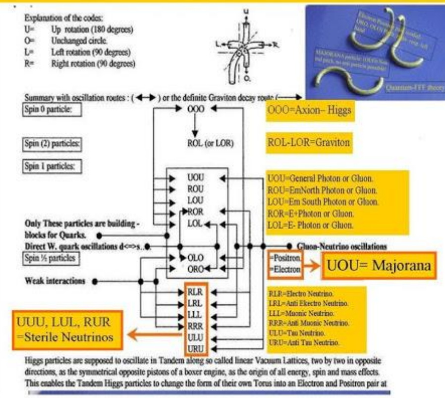
Figure 6, Single rigid string particles with much dualities, (stil undiscovered) described by only three hinges and 4x possible rotations of 90 degrees. (ULRO)
