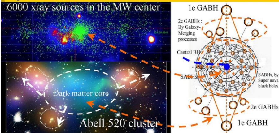
Figure 28, Non inertial Gravitating Dark Matter Black Holes and some specific astrophysical effects.
