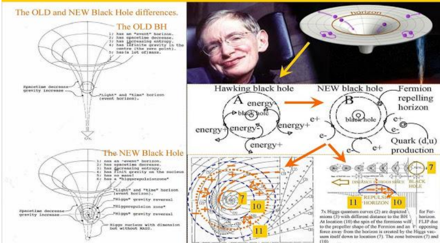
Figure 33, Negative charged Black hole at the outside, positive at the inside originated by the chiral vacuum.
