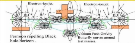
Figure 20, Secondary and Tertiary Dual BH HH systems.
