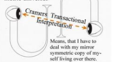
Figure 36: Schrodinger's cat problem is solved by Cramer's TI. No human eye is needed for cats.
