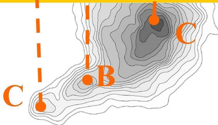
Figure 21, BOK Nebula ESO 9934.
