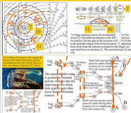
Figure 30, Super Nova Starspot Black Holes forming small Herbig Haro systems.
