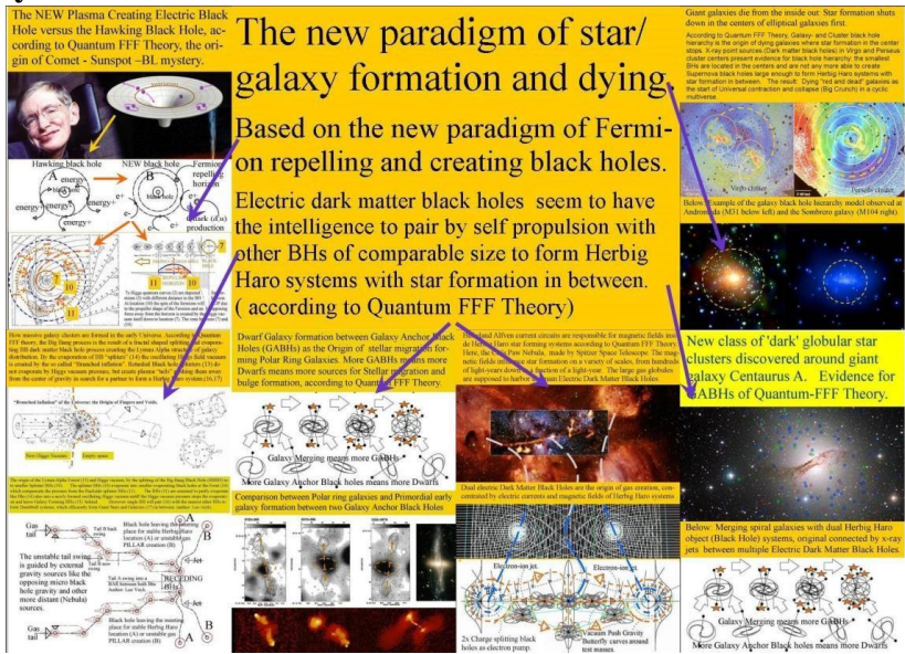
Figure 17, The new paradigm.
