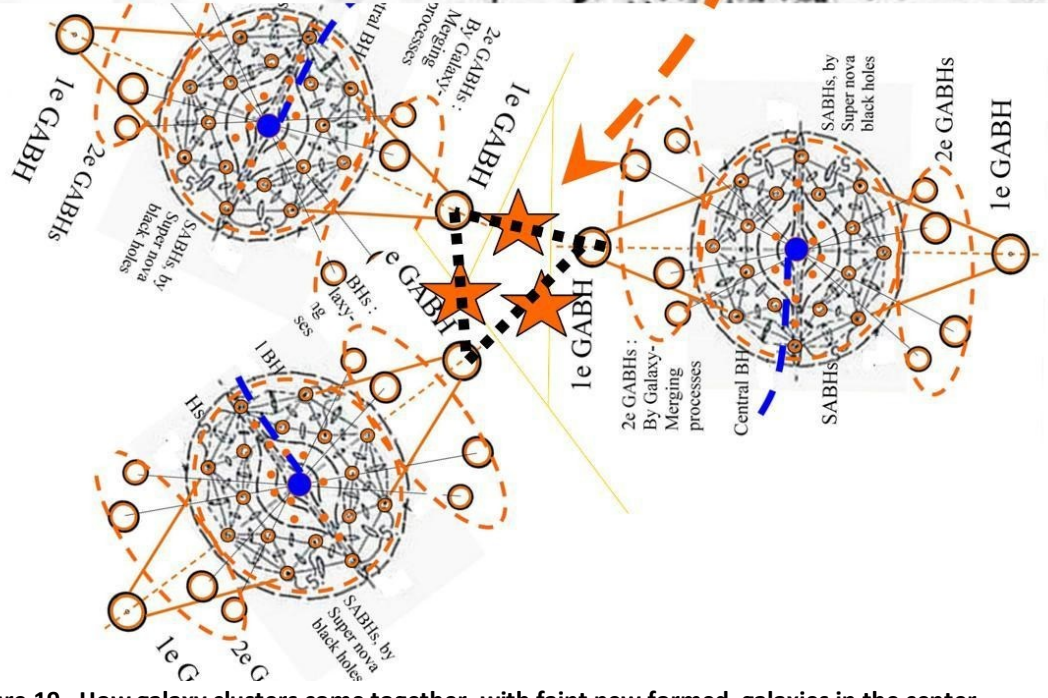
Figure 19. How galaxy clusters come together, with faint new formed galaxies in the center.
