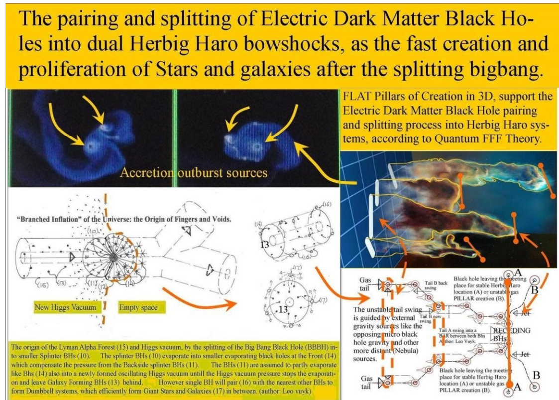
Figure 13, Examples of HH objects and dual DMBH pairing
