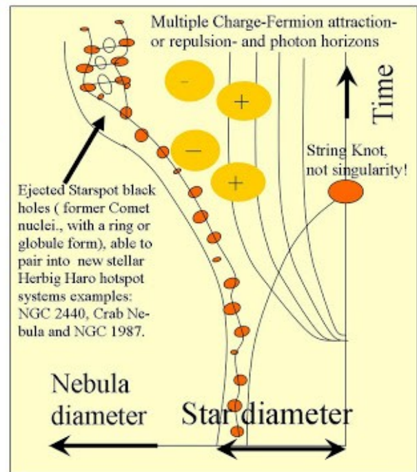
Figure 25, Super Nova Starspot Black Holes forming small Herbig Haro systems.
