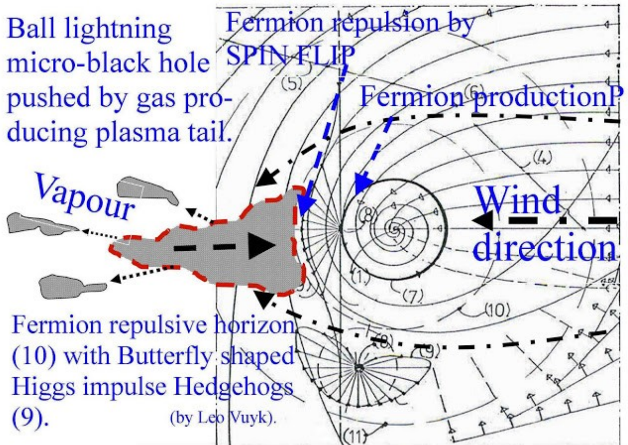
Figure 30., Details of vacuum synchrotron motion around a black hole with plasma creation and tail.
