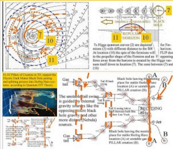
Figure 25, Super Nova Starspot Black Holes forming small Herbig Haro systems.
