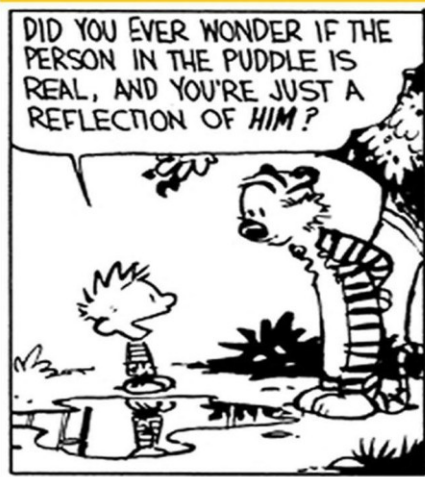
Figure :A Schrodinger's cat problem is solved by Cramer's TI. No human eye is needed for cats
