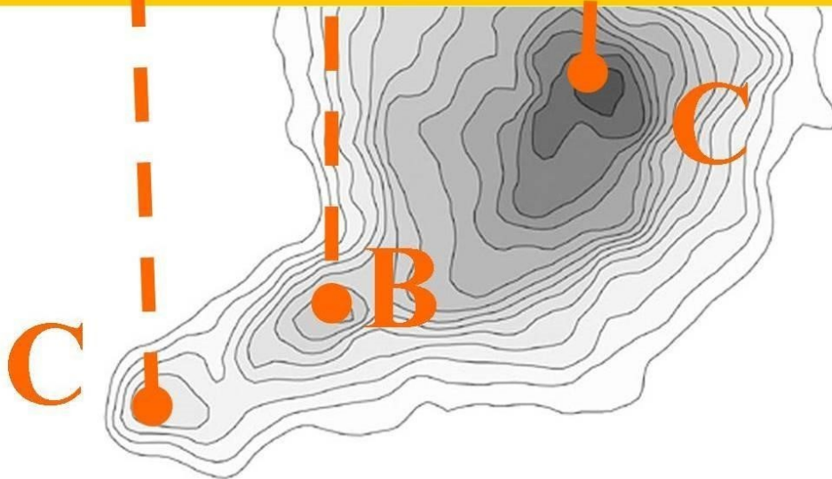
Figure 16, BOK Nebula ESO 9934.
