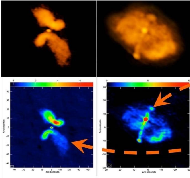
Figure 14, Abundance of X shaped radio sources.
