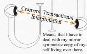
Figure :A Schrodinger's cat problem is solved by Cramer's TI. No human eye is needed for cats
