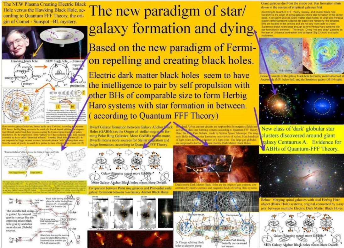
Figure 12, The new paradigm.
