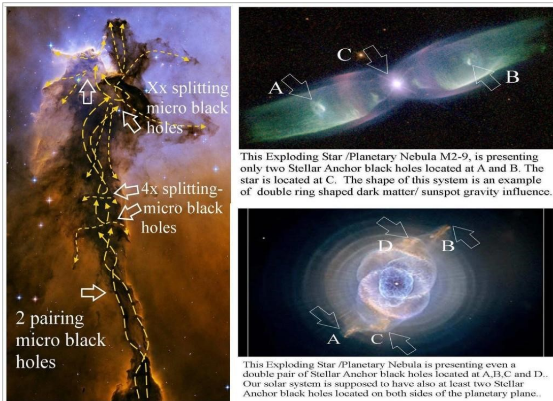
Figure 7, The Spire Eagle nebula, with two Planetary nebula, examples of the importance of black holes in the universe.
