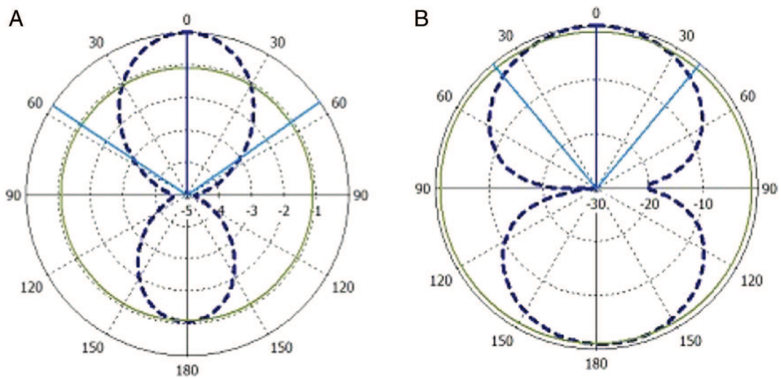
Figure 4: Radiation patterns of the antenna at 2.4 GHz: (A) \phi = 0 deg. plane and (B) \phi = 90 deg. plane.
