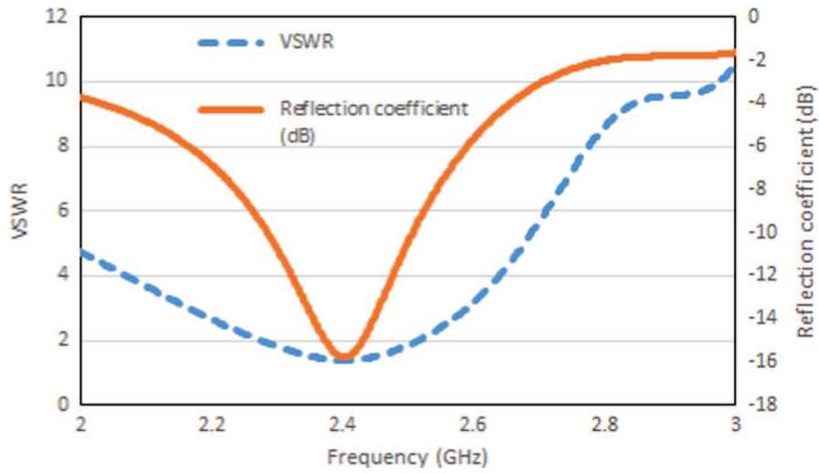
Figure 3: VSWR and reflection coefficient of the antenna.
