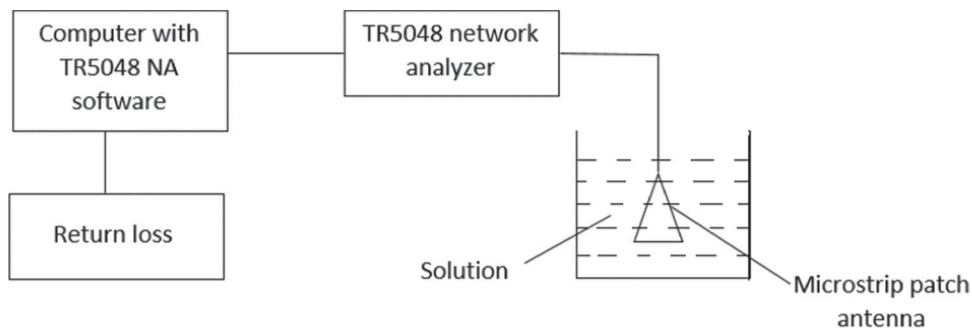
Figure 5: Measurement setup.
