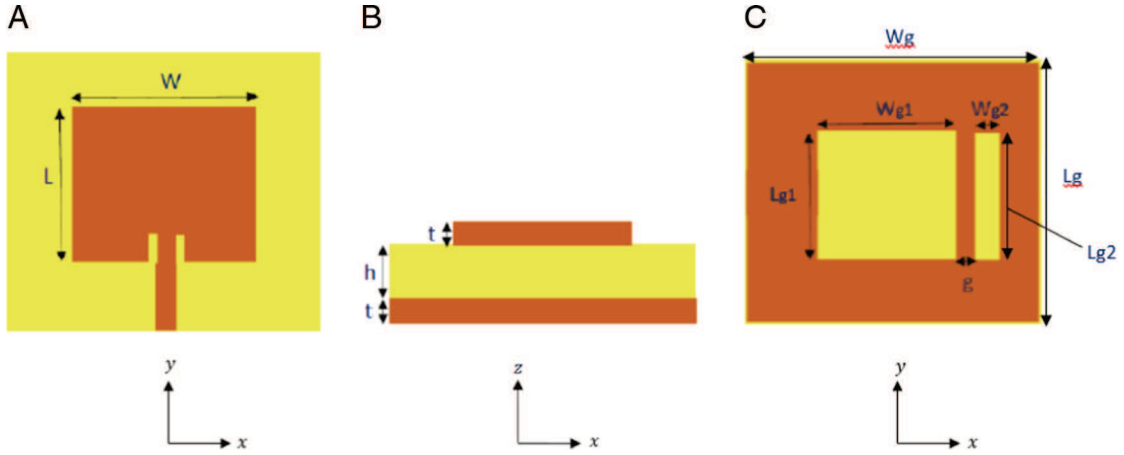
Figure 1: Antenna geometry: (A) top view, (B) side view, and (C) bottom view.
