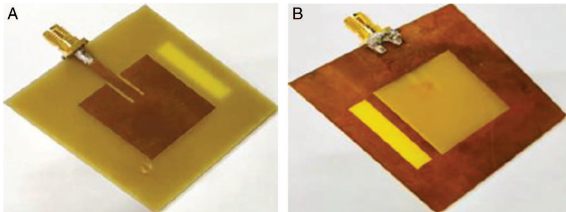
Figure 2: Fabricated antenna: (A) top view and (B) bottom view.
