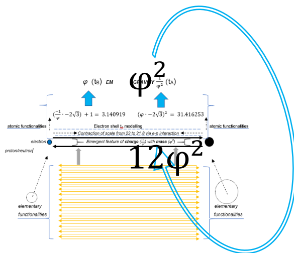
Paper 5, figure 4: \varphi^2 \gg 12 \varphi^2, \varphi^2 \gg (\varphi \cdot -2\sqrt{3})^2 , a process of the CMBR.
