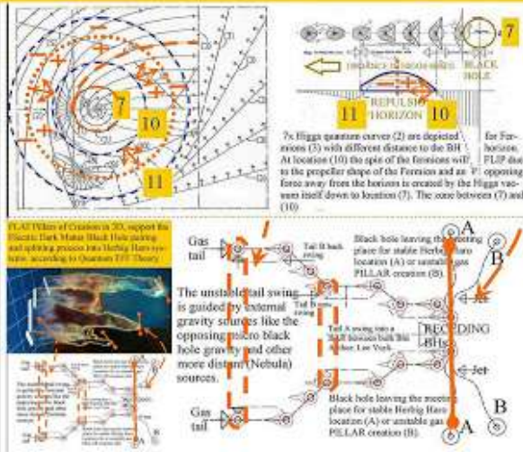
Figure 26, Super Nova Starspot Black Holes forming small Herbig Haro systems.
