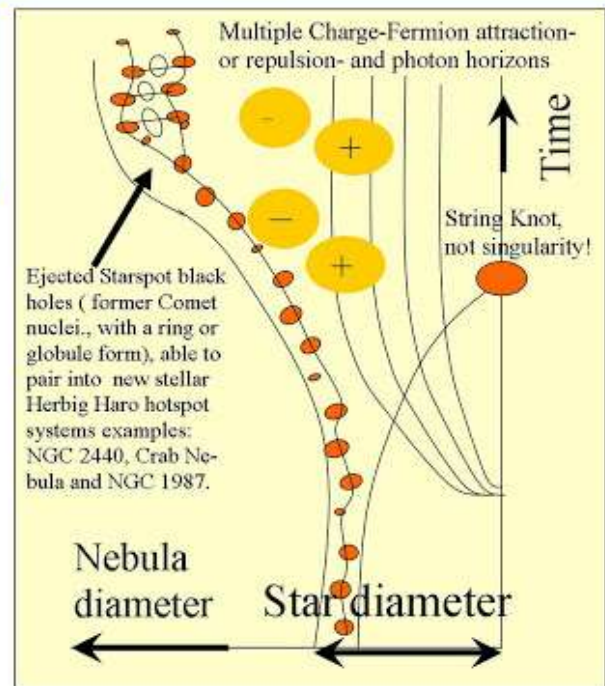
Figure 26, Super Nova Starspot Black Holes forming small Herbig Haro systems.
