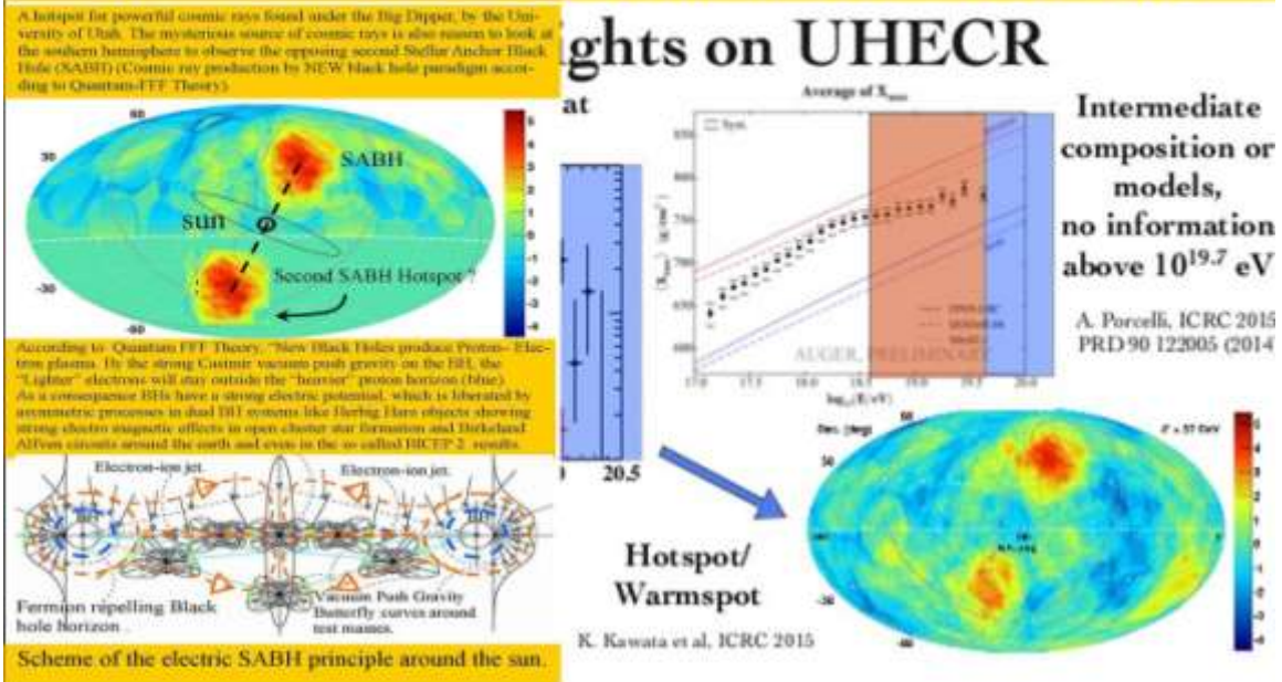
Figure 4, UHECR = Ultra High Energy Cosmic Radiation by A Porcelli ICRC 2015. PRD90122005 (2014) and A. Kawata et al. ICRC 2015.
