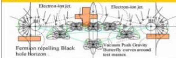
Figure 15, Secondary and Tertiary Dual BH HH systems.
