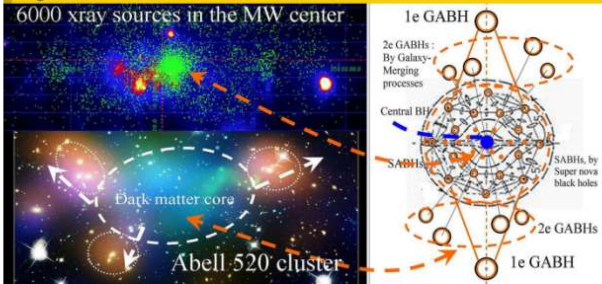
Figure 23, Non inertial Gravitating Dark Matter Black Holes and some specific astrophysical effects.
