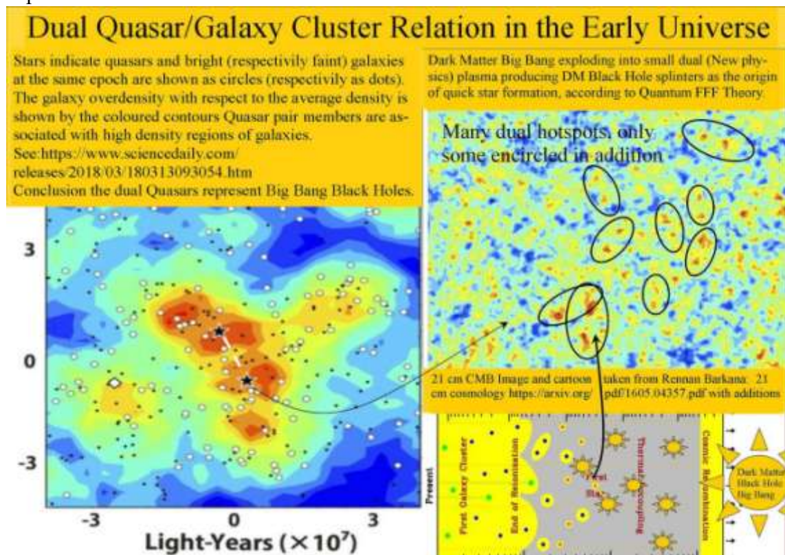
Figure 8, Dual Quasar/ Galaxy and Cluster forming relation in the early universe after Dark Matter Black Hole nuclear Big Bang splitting.
