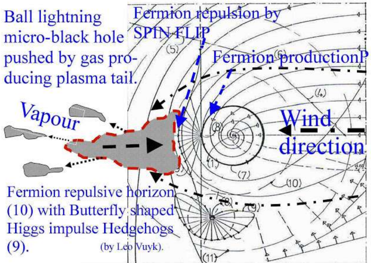
Figure 22, Details of vacuum synchrotron motion around a black hole with plasma creation and tail.
