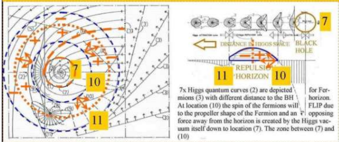
Figure 9, Principle of Fermion repulsion around a black hole according to Quantum FFF theory..
