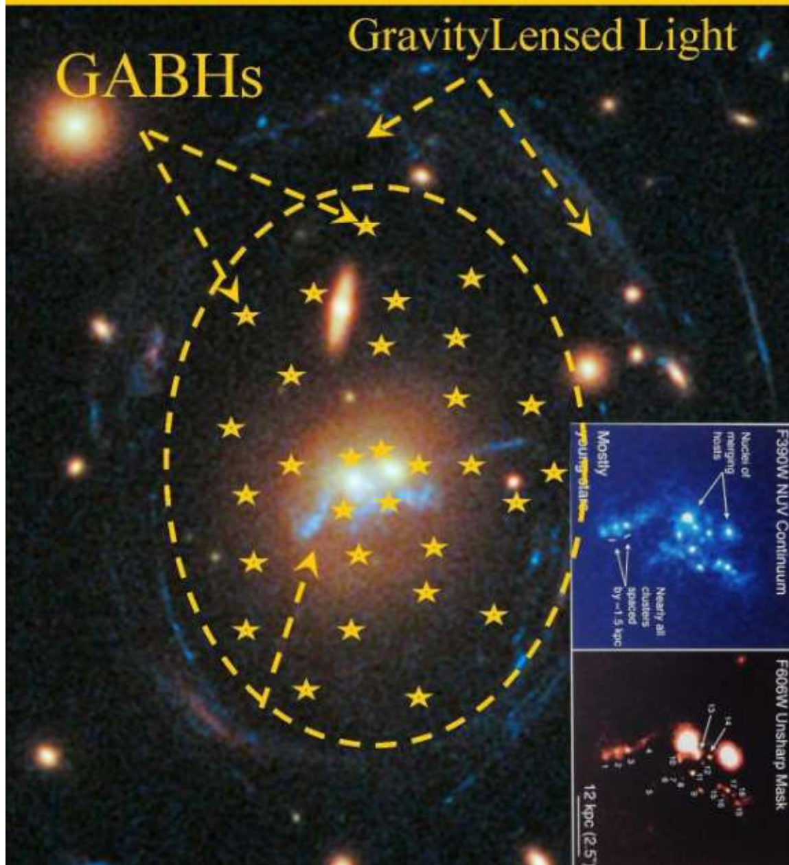
Figure: 11, Gravity lensed light through central hole in the globular Shell of Dark matter Black Holes or Galaxy Anchor Black Holes ( GABHs). The absence of GABHs in the centre is supposed to do the job.
