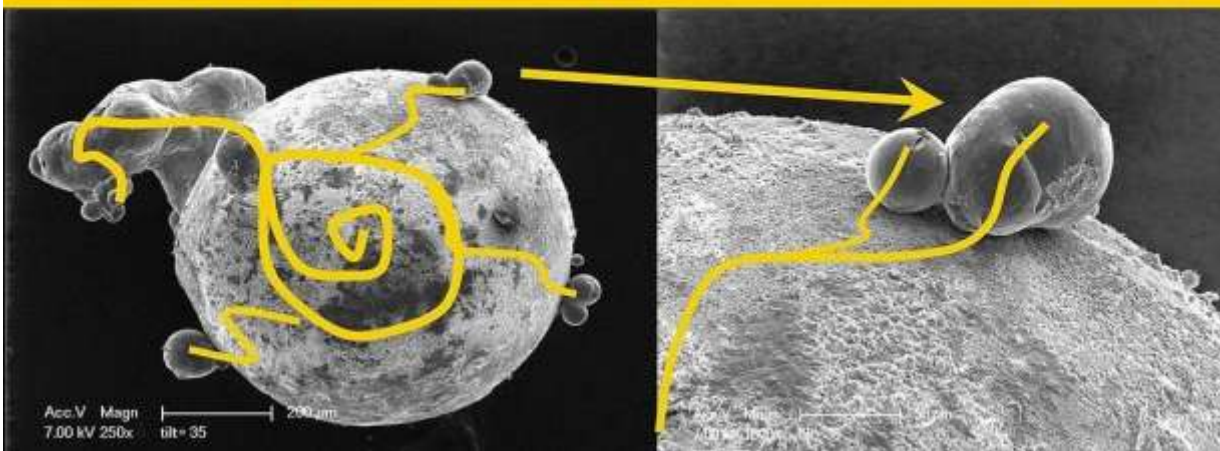
Figure 24. Magnetic Interference microscopic Higgs black holes, ( quantum Knots) with heating effects in silicon and as CERN LHC UFO dust particles.
