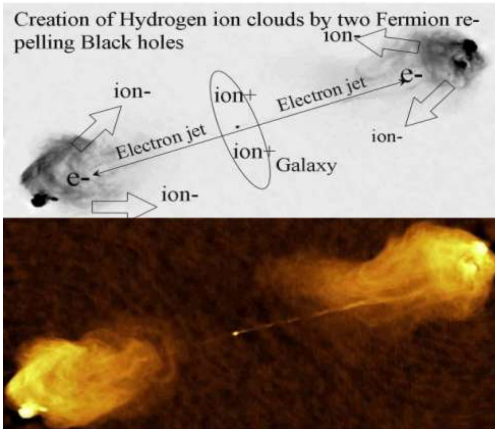
Figure 6, Cygnus A, equipped with Galaxy Anchor Black Holes (GABHs) clear electron jets and Hotspots, showing ionized gas production.
