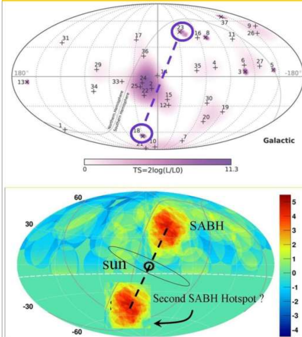
Figure: 10, 9-july 2014. first evidence for the first Solar Anchor Black Hole. (SABH) A hotspot with powerful cosmic rays found under the Big Dipper, by the University of Utah. Now ( 2017) however the southern counterpart ( the second SABH hotspot) is found, see figure 1.
