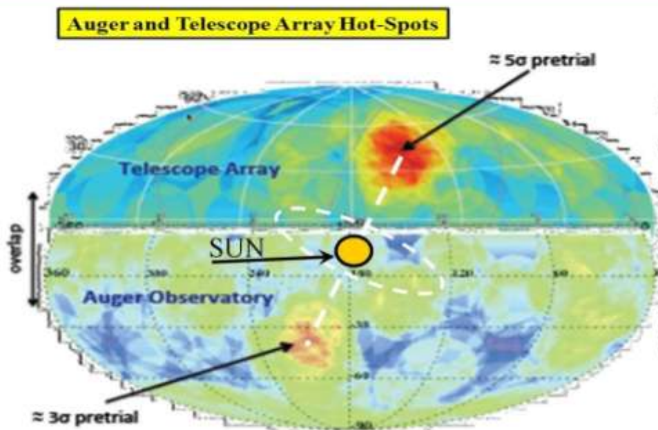
Figure 1, Two Stellar Anchor Black Holes (Herbig Haro hotspots) at both polar sites of the sun. According to Quantum FFF Theory.
