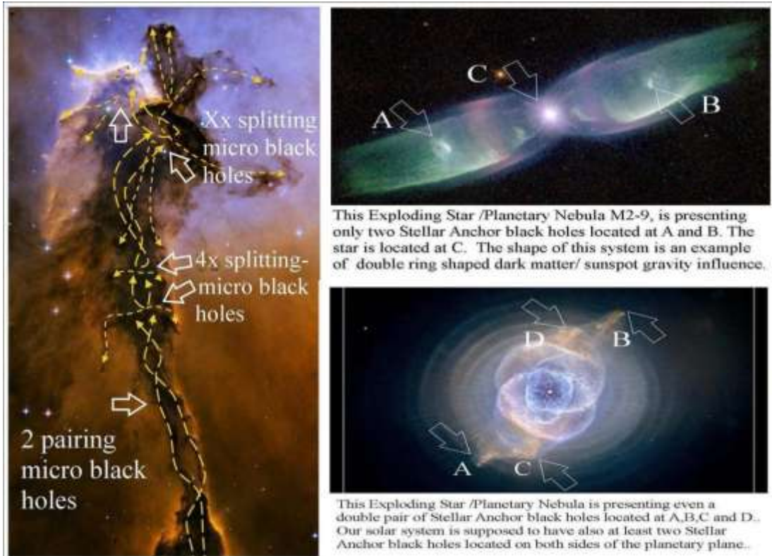
Figure 7, The Spire Eagle nebula, with two Planetary nebula, examples of the importance of black holes in the universe.
