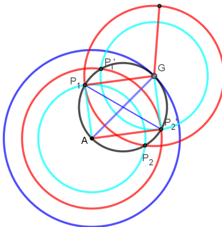
Fig. 4. Circles are drawn with AG as diameter. From the opposite ends A and G as centers, circles are drawn with radii r_1 and r_2 . The points of intersection are marked as P_1, P_2, P_1', P_2' . Cyclic quadrilateral AP_1GP_2' is drawn.
